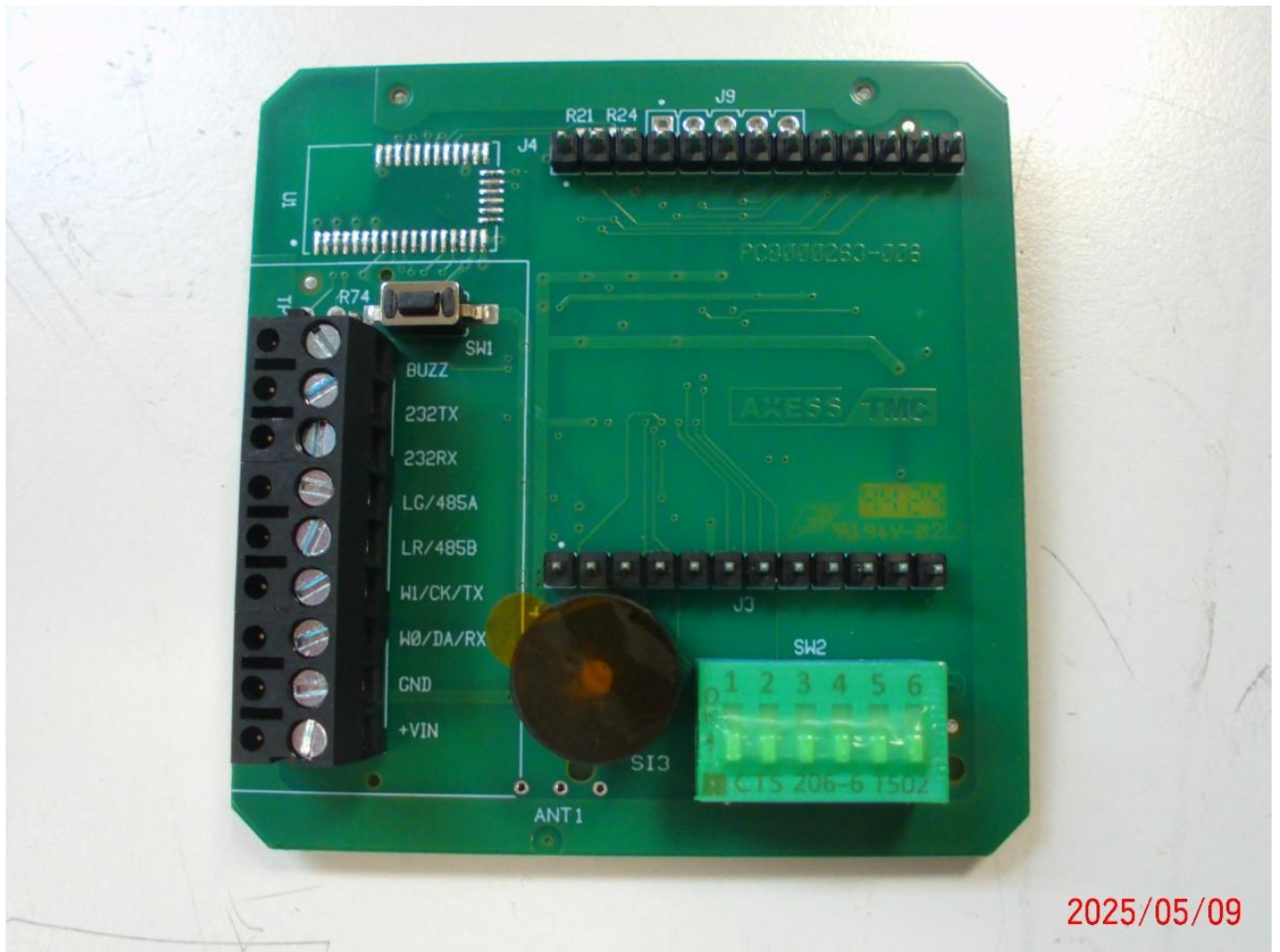
Fig. 4.Board PCB000263-006, side one (radio module PCB000411_002 dismountled)
