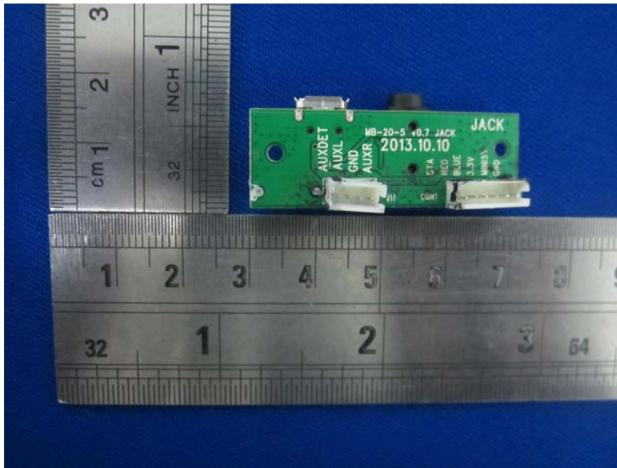
EUT- Charge and Audio Board Bottom View
