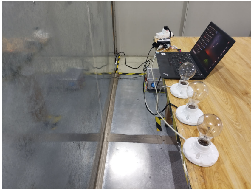
Conducted Emissions (Left View)
