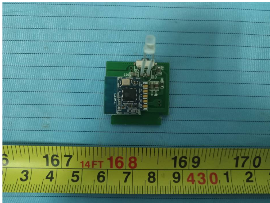
EUT –Wifi Module Top Sheilding off View
