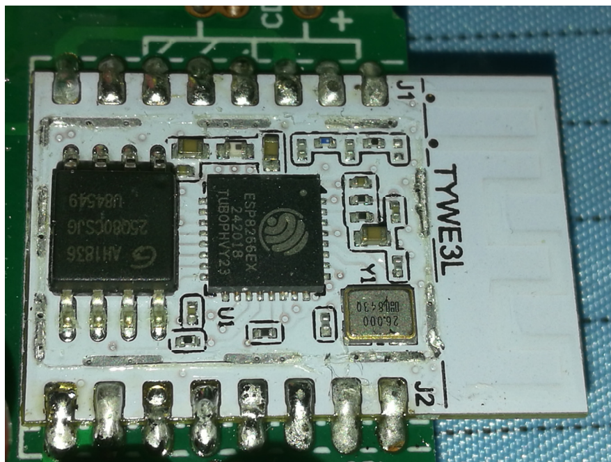
EUT –Module Sheilding off View
