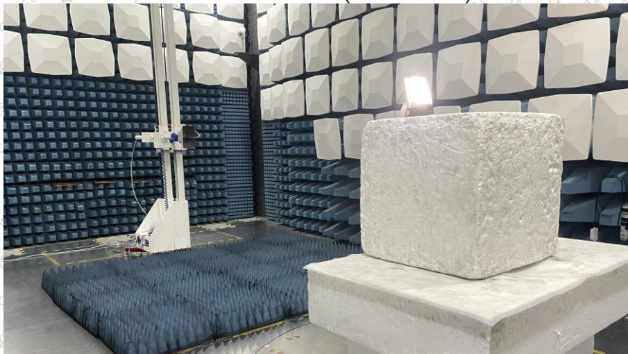
Radiated Emissions (Above 1 GHz)
