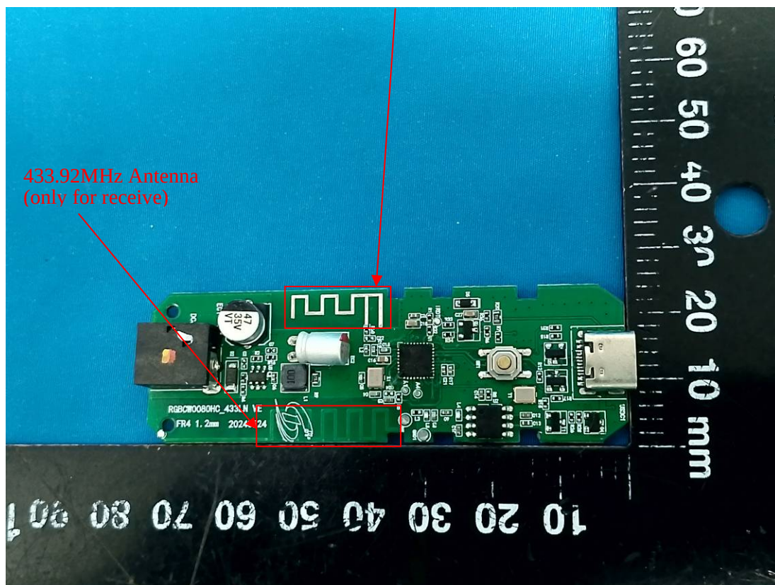
Wifi Antenna
