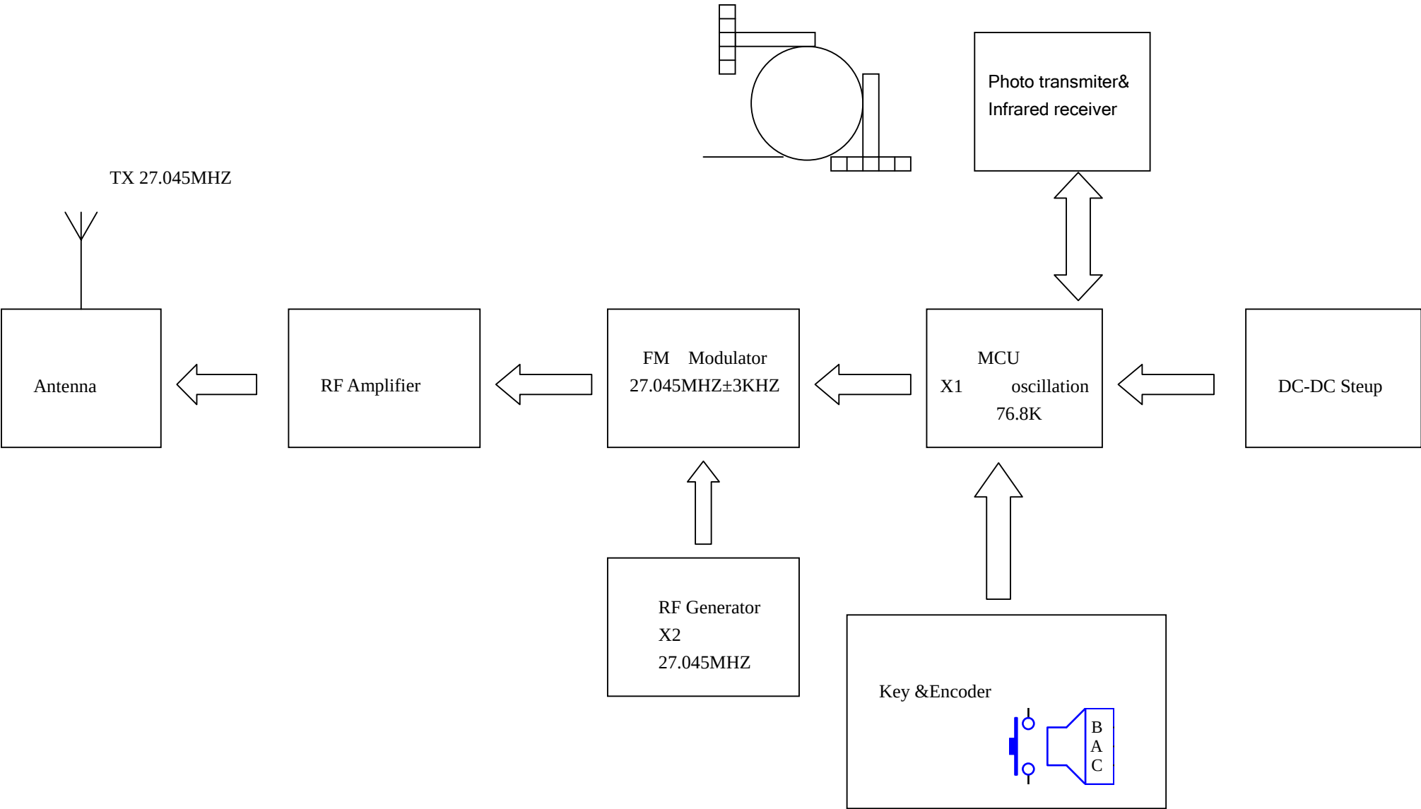
DS-2009 Block Diagram
