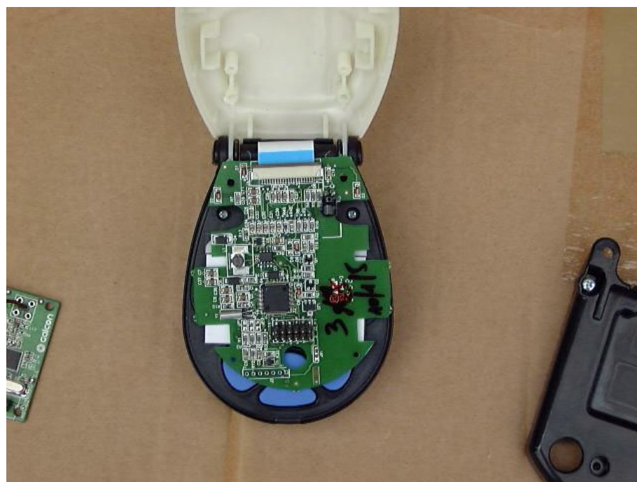
Figure 4 PCB Side 1 Side 2
