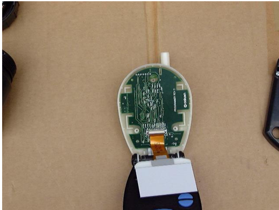
Figure 2 PCB In Case
