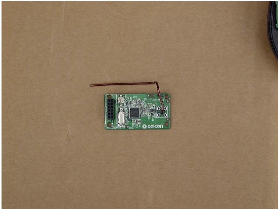
Figure 5 PCB 2 Side 1
