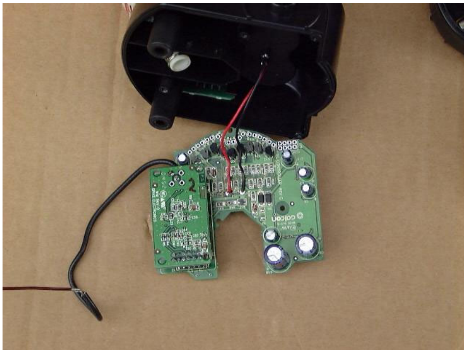
Figure 2 PCB 1 Side 1
