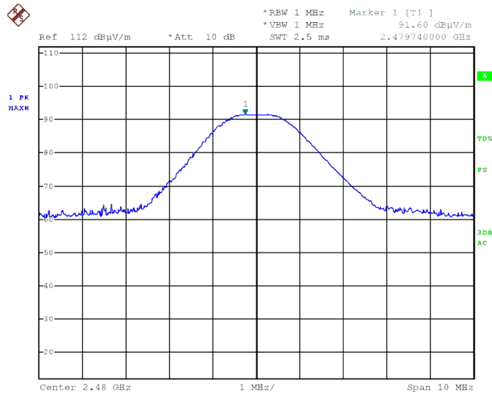
Figure 17 2480.0 MHz – Vertical
