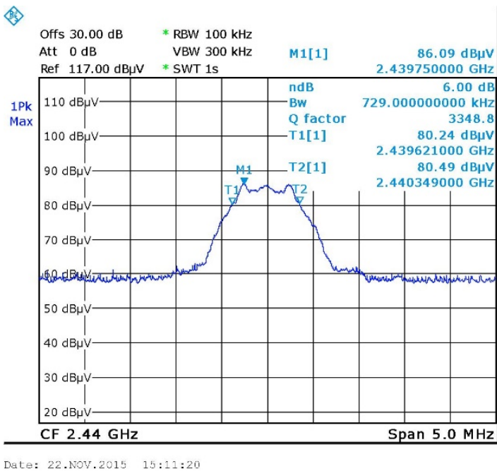
Figure 9. 2440.0 MHz
