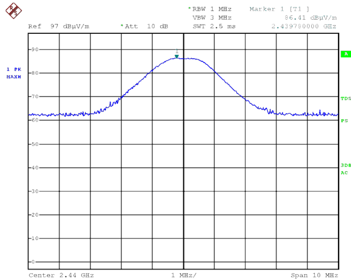
Figure 15 2440.0 MHz – Vertical
