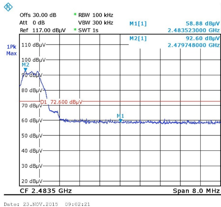
Figure 22 —Upper Band Edge
