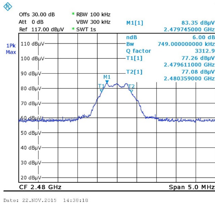
Figure 10. 2480.0 MHz
