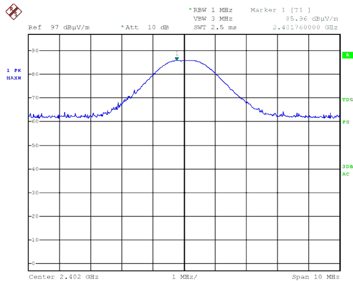
Figure 13 2402.0 MHz – Vertical
