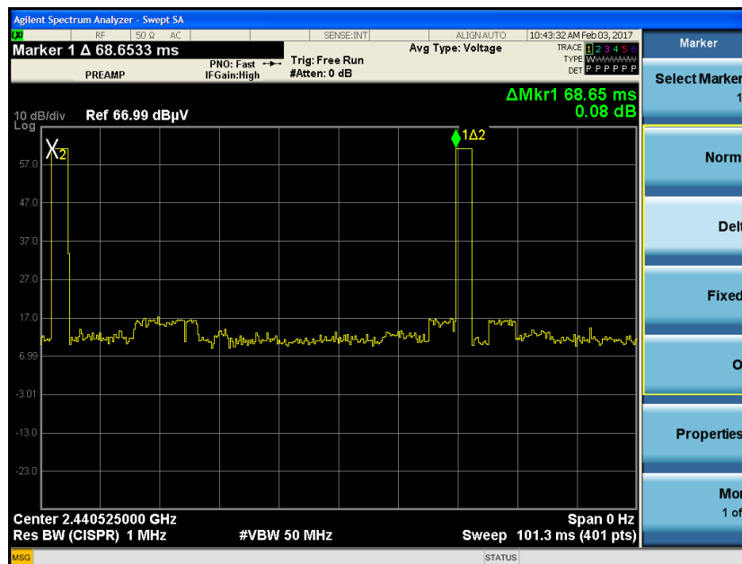
Pulse Train
