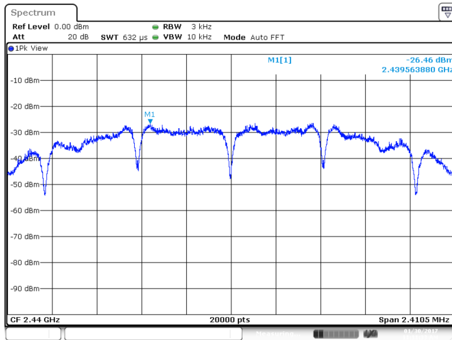
Middle Channel PSD
