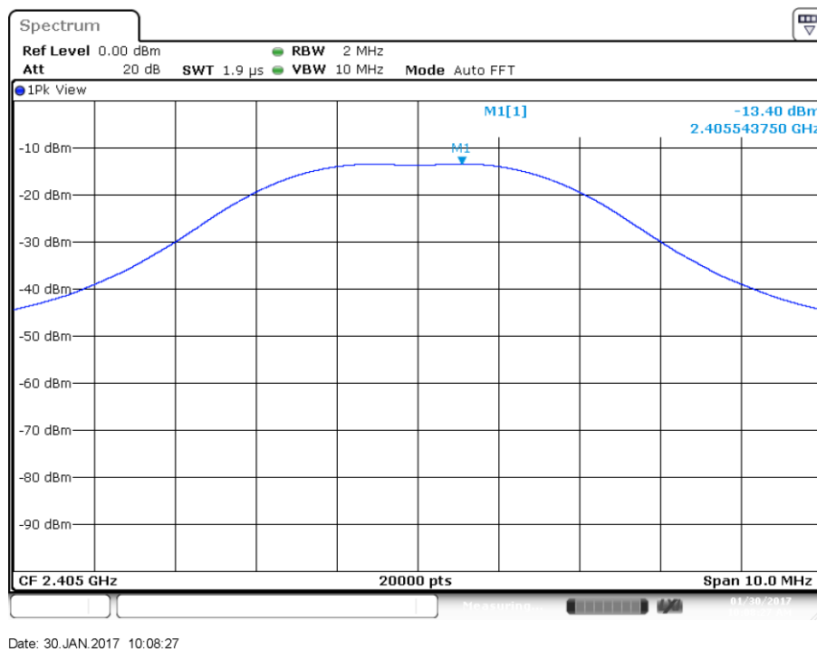
Low Channel Peak Output Power
