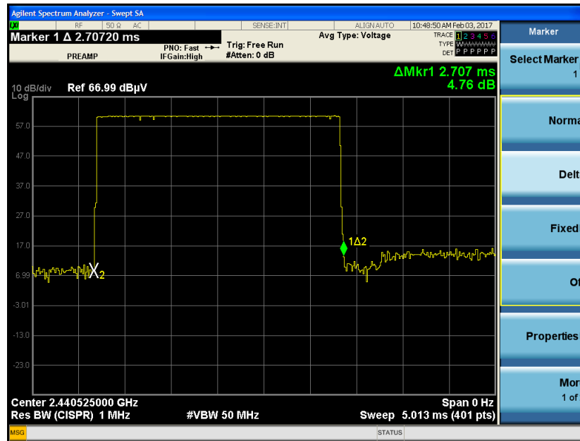
Single pulse
