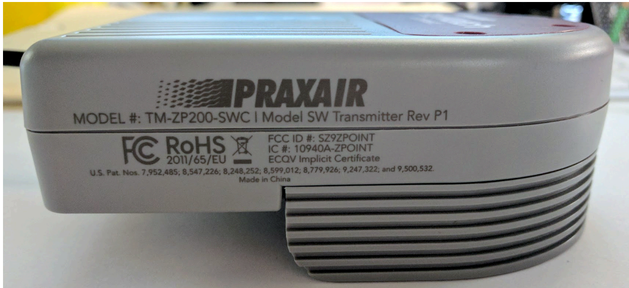
Right Side
