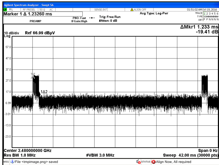
Individual Pulse
