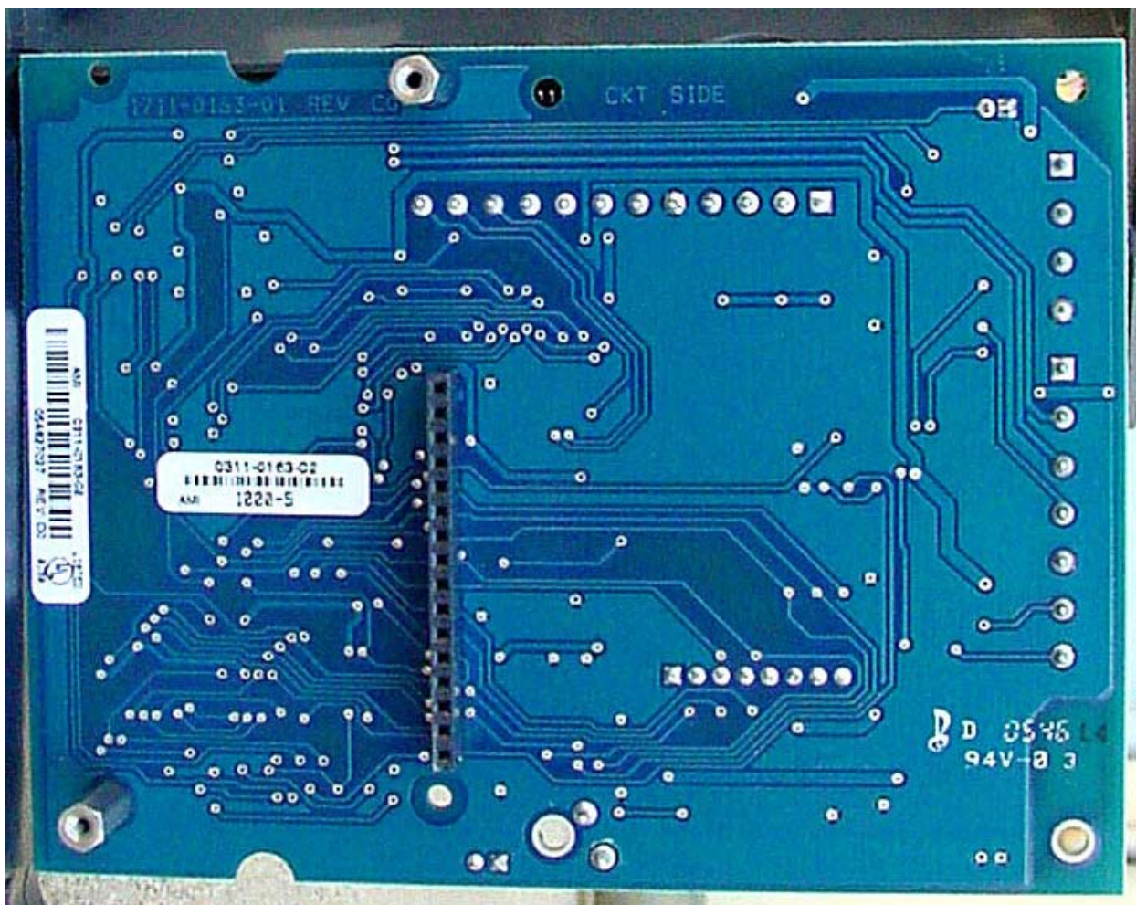
RM Board – Rear
