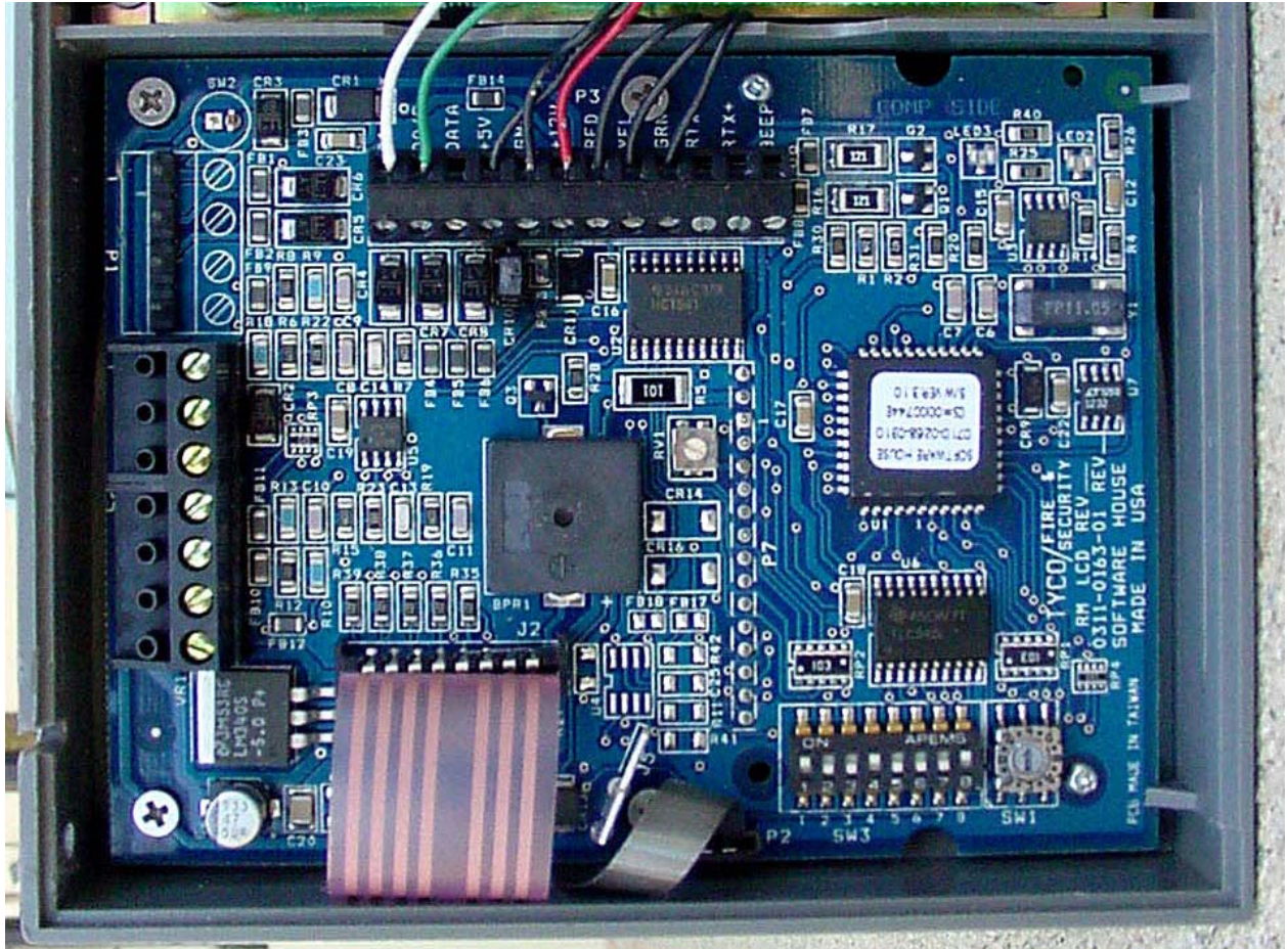
RM Board – Front
