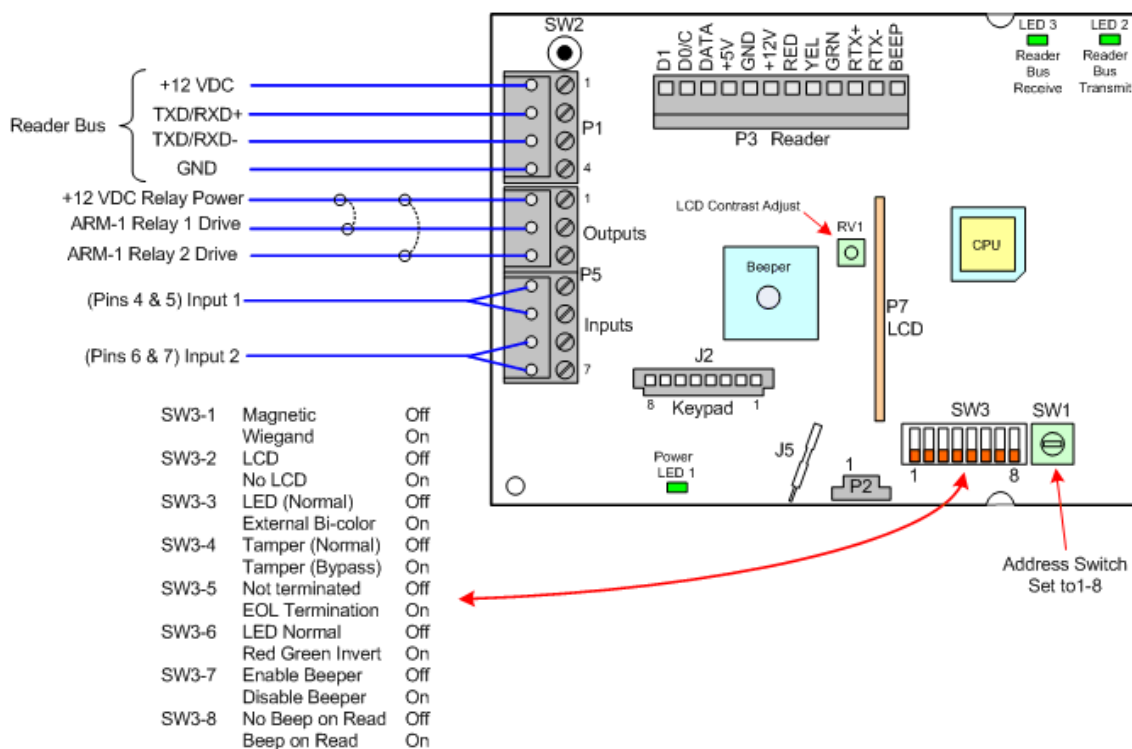
FIGURE 3. RM-4 Wiring Requirements
