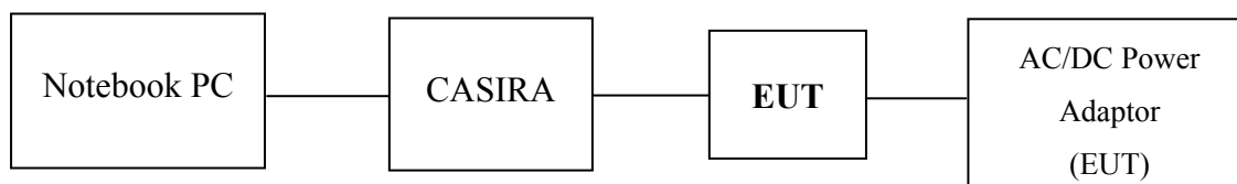
Fig. 2-1 Configuration of Tested System
