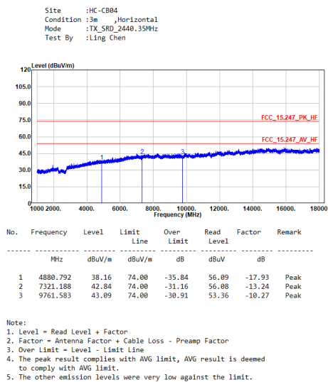
TX_SRD_2440.35MHz_H
