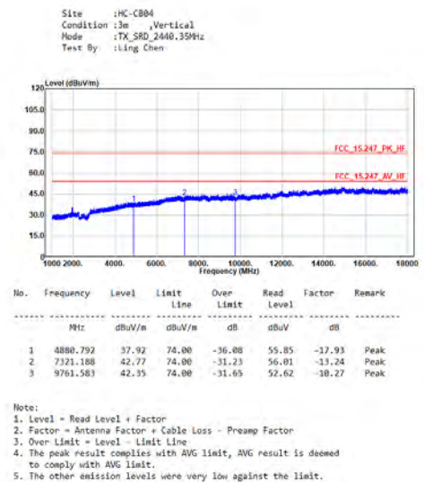
TX_SRD_2440.35MHz_V
