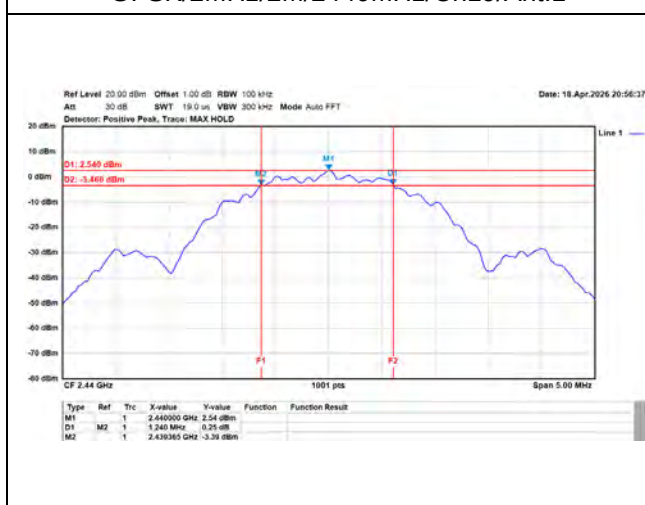
GFSK/2MHz/2M/2440MHz/Ch19/Ant.1
