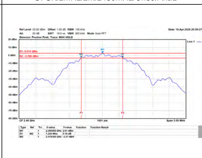
GFSK/2MHz/2M/2480MHz/Ch39/Ant.1
