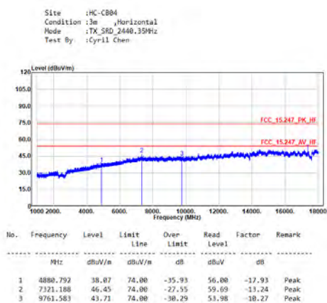
TX_SRD_2440.35MHz_H
