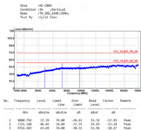
TX_SRD_2440.35MHz_V
