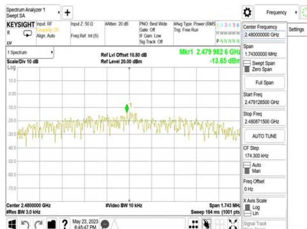
PSD_BLE 2M_HighCH39-2480MHz
