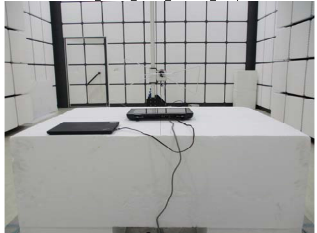
Part 15.247 WLAN Radiated variant Setup
