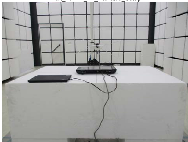
Part 15.247 LE Radiated variant Setup
