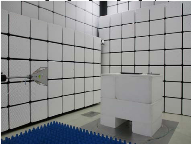
Part 15.247 WLAN Radiated Setup
