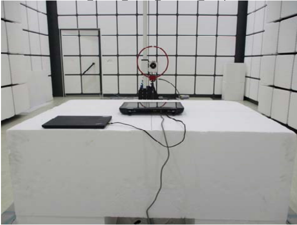
Part 15.247 WLAN Radiated variant Setup
