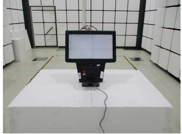
P15.225 NFC Radiated Setup
