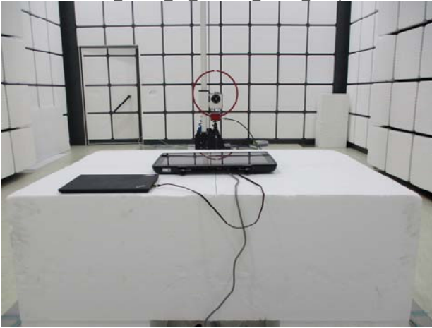
Part 15.247 LE Radiated Setup
