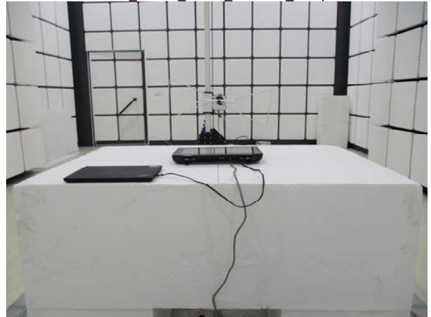
Part 15.407 WLAN Radiated Setup
