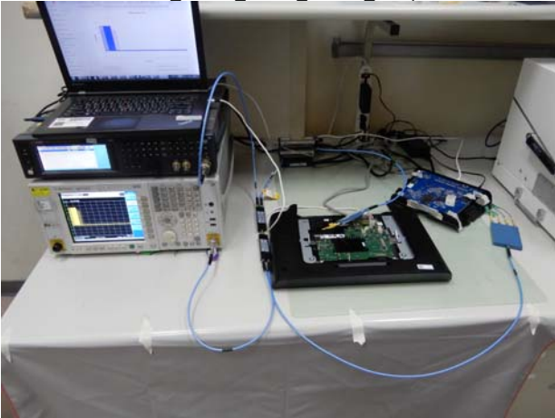
Part_15.407_WLAN_Normal_Setup
