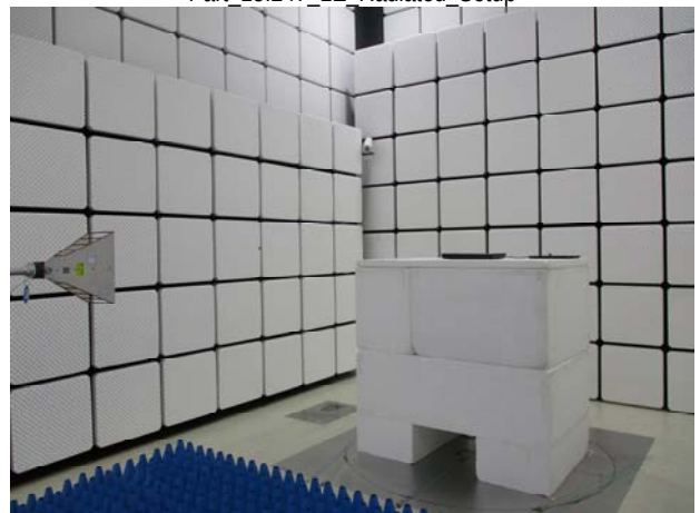
Part 15.247 LE Radiated Setup
