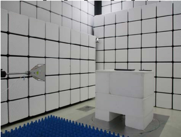
Part 15.407 WLAN Radiated variant Setup
