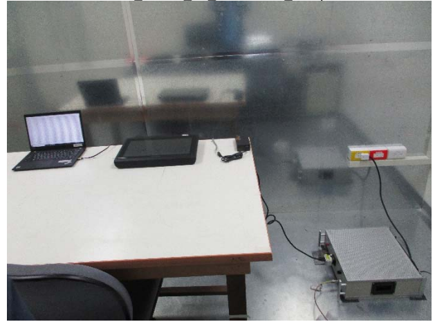
Part 15.247 LE Conduction Setup
