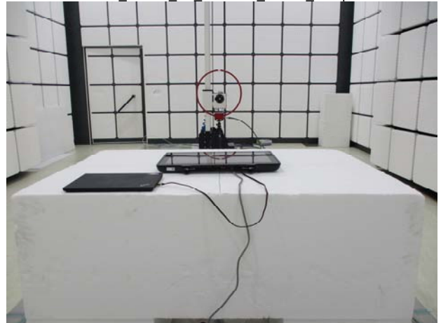
Part_15.247_BT_Radiated_variant_Setup
