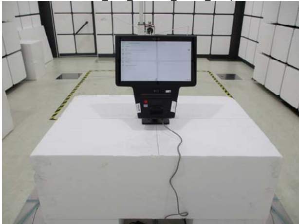
P15.225 NFC Radiated variant Setup
