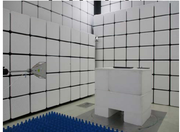
Part 15.247 BT Radiated variant Setup
