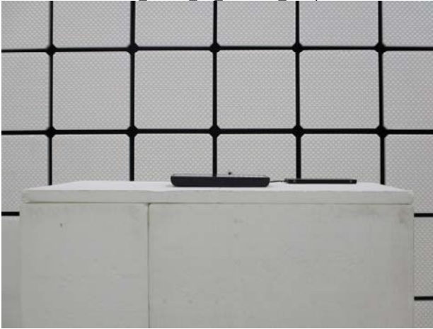
Part_15.247_BT_Radiated_variant_Setup
