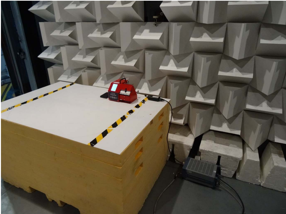
Conducted emission
