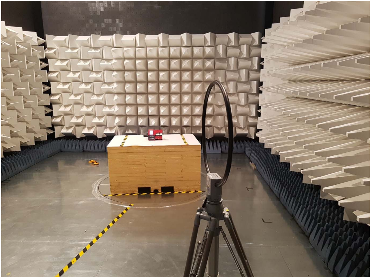
Radiated < 30MHz
