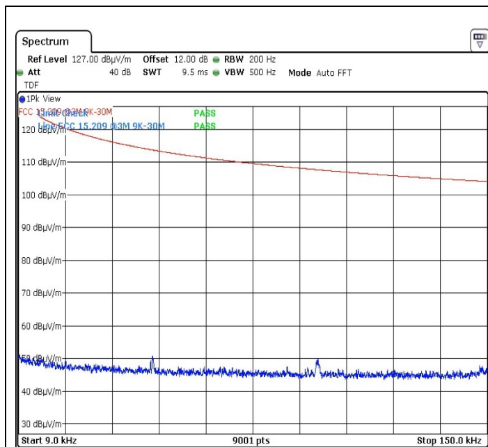
Radiated Emissions, 9 – 150 kHz Bottom Channel
