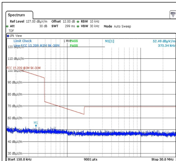
Radiated Emissions, 150 kHz – 30 MHz Bot Ch
