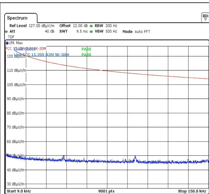
Radiated Emissions, 9 – 150 kHz Top Channel
