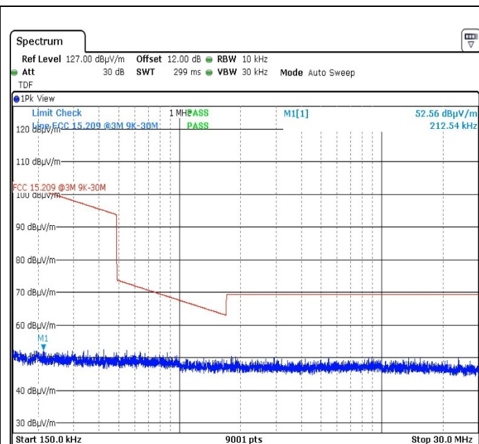
Radiated Emissions, 150 kHz – 30 MHz Top Ch
