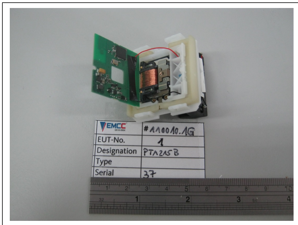
Photograph A4-2: EUT#1, connection from battery to PCB
