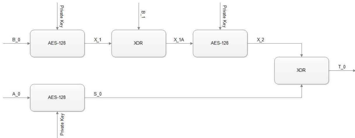
Figure 60 – Authentication algorithm sequence
