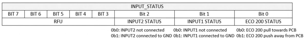
Figure 15 – INPUT_STATUS structure
