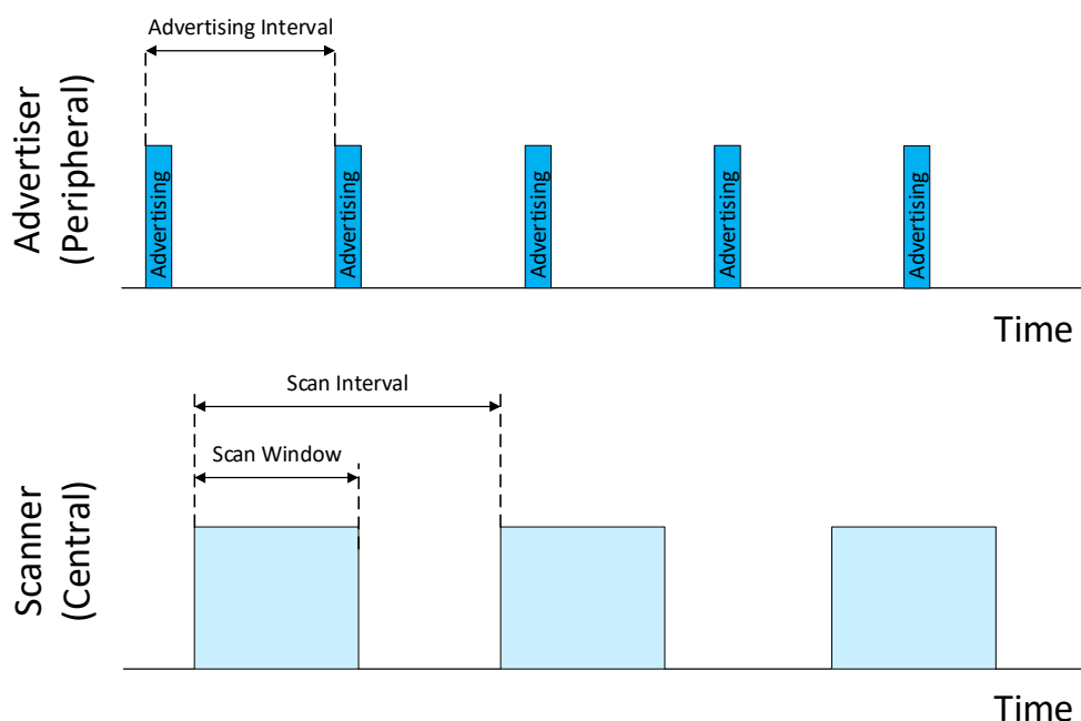
Figure 57 – Scanning parameters
