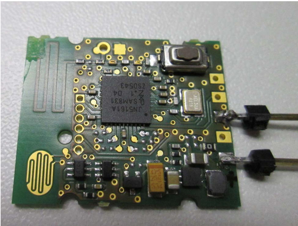
Photo A2-1: EUT variant #1 – Top view
