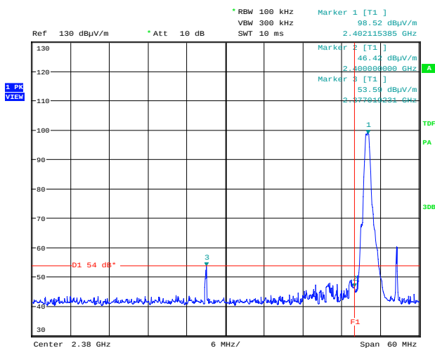
Band-Edge Compliance – Lower Edge Variant #2 Channel: low
