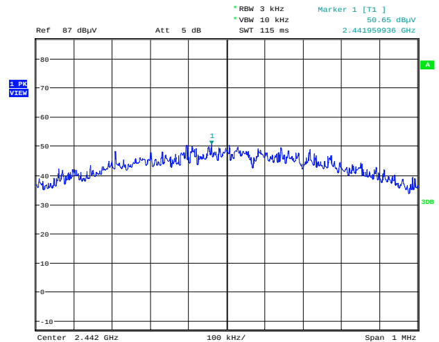
Power Spectral Density Variant #3 Channel: middle
