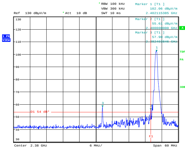
Band-Edge Compliance – Lower Edge Variant #1 Channel: low
