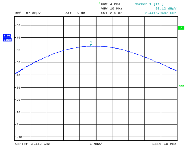
Fundamental emission output power Variant #3 Channel: middle
