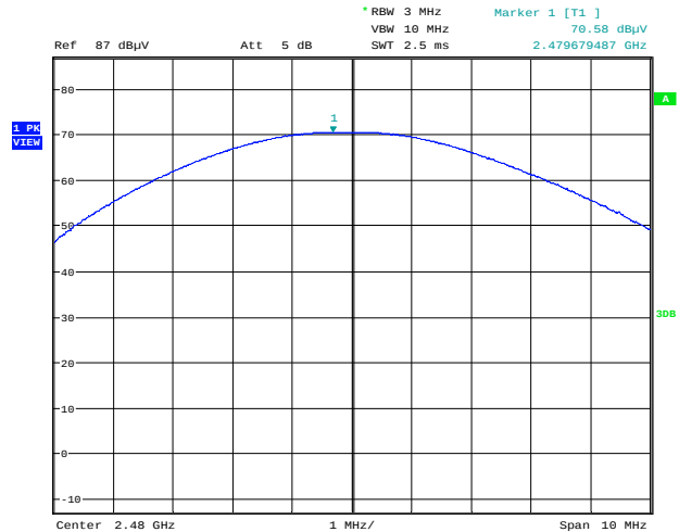
Fundamental emission output power Variant #2 Channel: high
