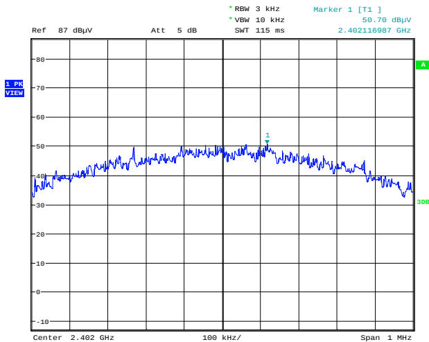
Power Spectral Density Variant #3 Channel: low
