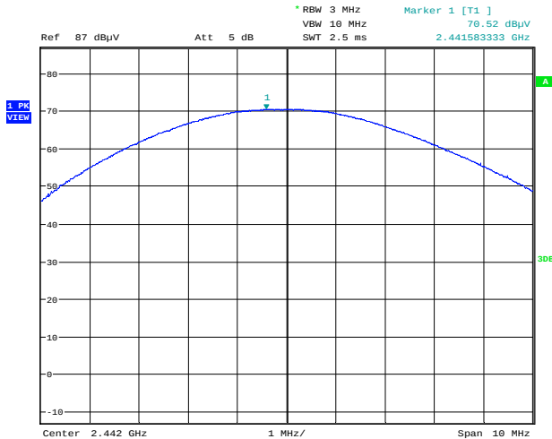
Fundamental emission output power Variant #2 Channel: middle
