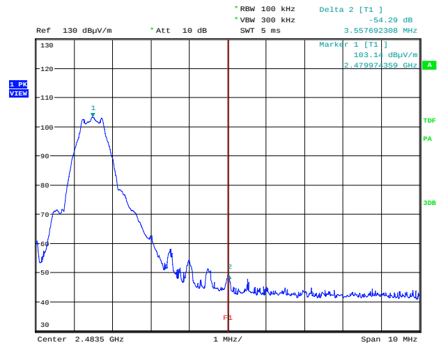
Band-Edge Compliance – Upper Edge Variant #1 – 100 kHz BW Channel: high
