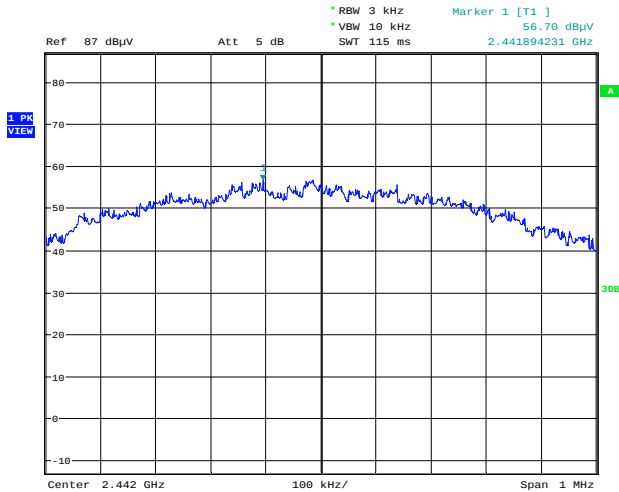
Power Spectral Density Variant #2 Channel: middle
