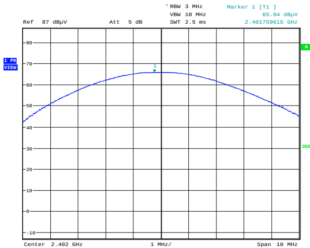
Fundamental emission output power Variant #3 Channel: low
