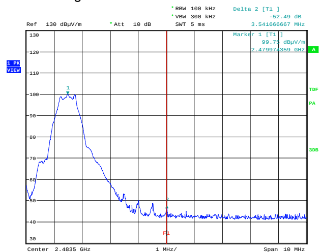
Band-Edge Compliance – Upper Edge Variant #2 – 100 kHz BW Channel: high
