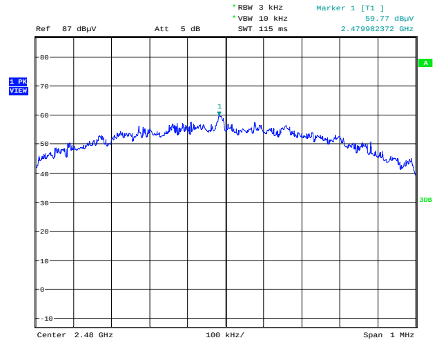
Power Spectral Density Variant #2 Channel: high
