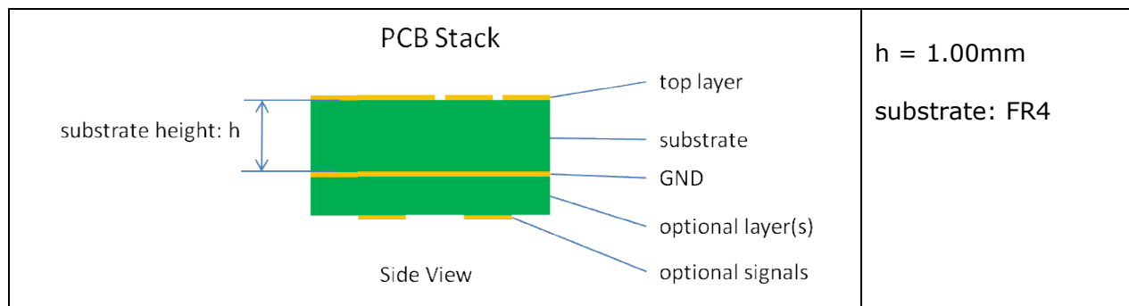
Figure 18 – PCB stack specification for meandered PCB antenna
