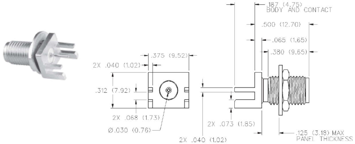
Figure 22 – RP-SMA-Female
