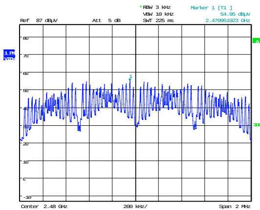
Power Spectral Density Variant #1 Channel: 26
