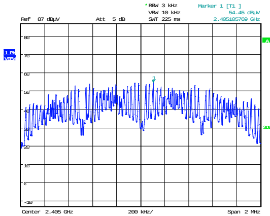
Power Spectral Density Variant #1 Channel: 11
