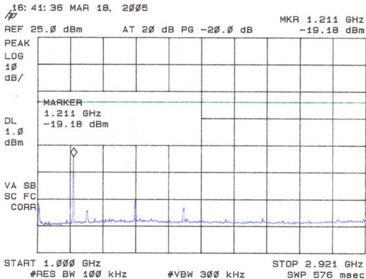
Figure 4j Antenna Conducted Spurious Emissions 15.247(c) (High Channel)
