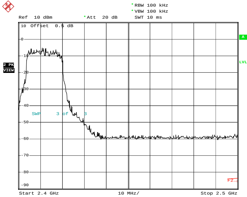
Plot No: 4.3
