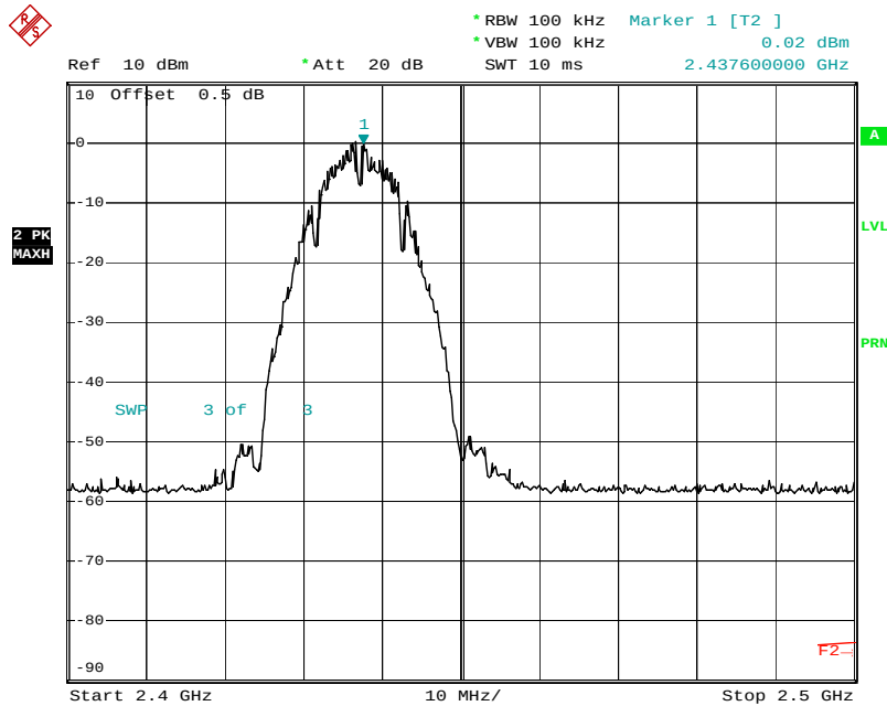
Plot No: 4.14
