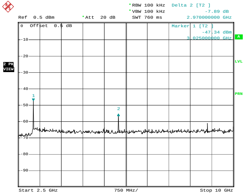
Plot No: 4.32
