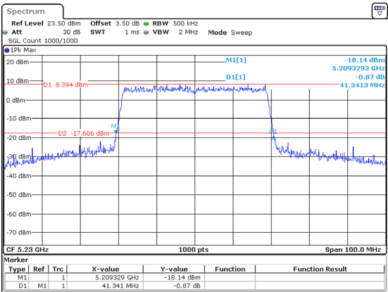
802.11ax40_5230MHz_RU_Full
