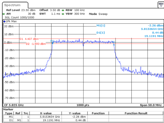
802.11ax20_5825MHz_RU_Full
