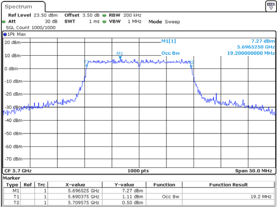
802.11ax20_5700MHz_RU_Full
