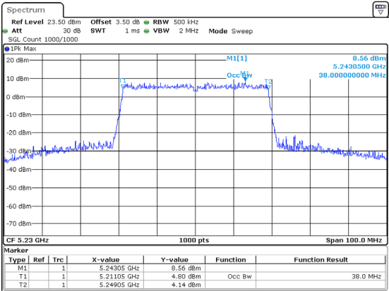
802.11ax40_5230MHz_RU_Full
