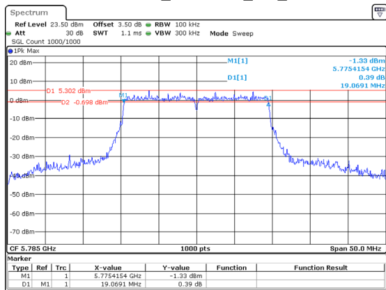
802.11ax20_5785MHz_RU_Full
