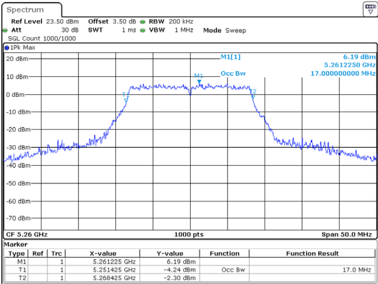
802.11a_5260MHz
