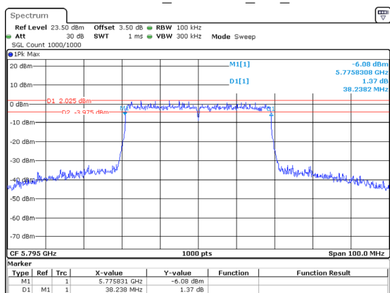
802.11ax40_5795MHz_RU_Full
