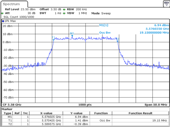
802.11ax20_5580MHz_RU_Full
