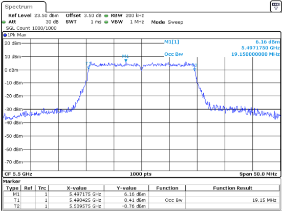
802.11ax20_5500MHz_RU_Full
