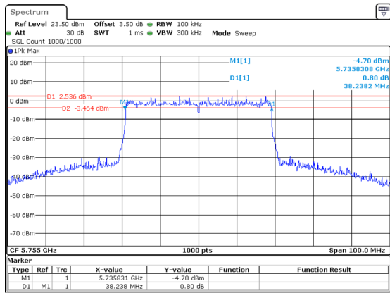
802.11ax40_5755MHz_RU_Full
