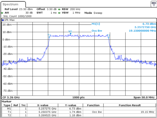
802.11ax20_5260MHz_RU_Full
