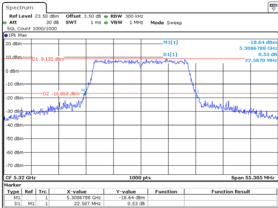
802.11ax20_5320MHz_RU_Full
