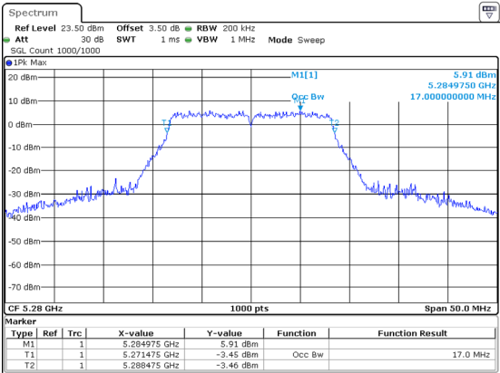
802.11a_5280MHz
