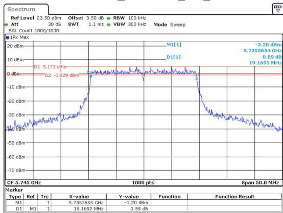
802.11ax20_5745MHz_RU_Full
