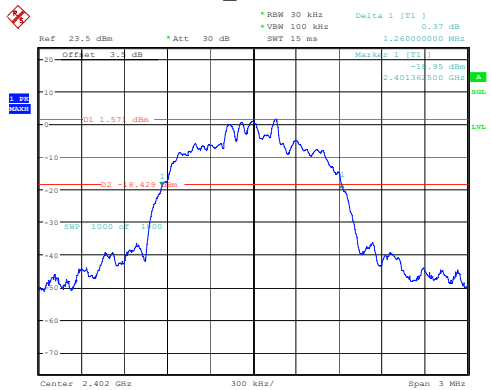
3DH1_Low 1.260MHz
