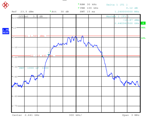
3DH1_Middle 1.260MHz
