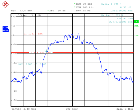
3DH1_High 1.256MHz
