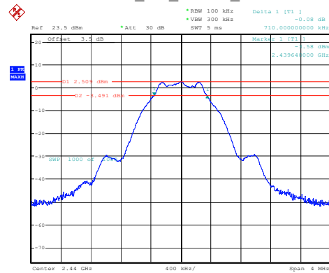
BLE_1M_Middle_Channel
