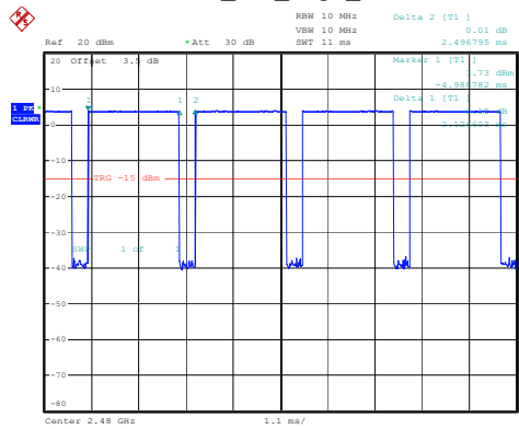
BLE_1M_High_Channel
