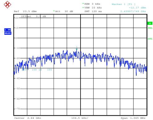
BLE_1M_Middle_Channel
