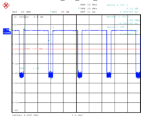
BLE_1M_Low_Channel
