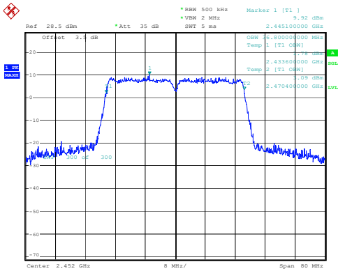
802.11n40_2452MHz
