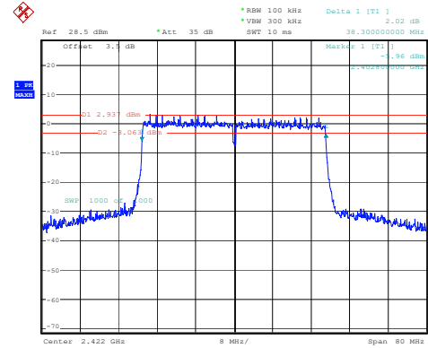
802.11ax40_2422MHz_RU_Full
