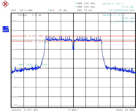
802.11n40_2437MHz
