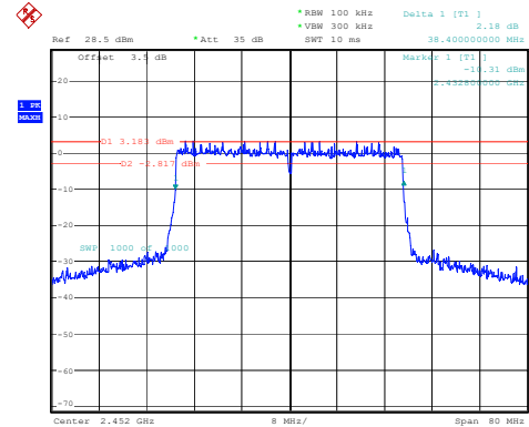
802.11ax40_2452MHz_RU_Full
