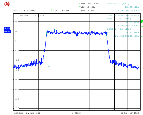
802.11ax40_2422MHz_RU_Full
