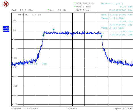
802.11ax20_2412MHz_RU_Full
