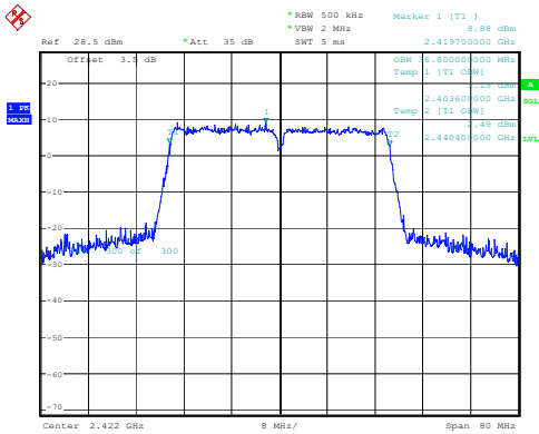
802.11n40_2422MHz
