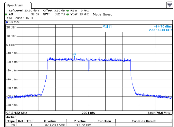
802.11ax40_2422MHz_RU_Full
