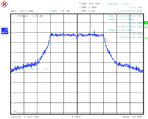
802.11g_2462MHz
