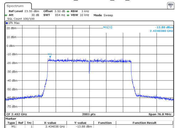
802.11ax40_2452MHz_RU_Full
