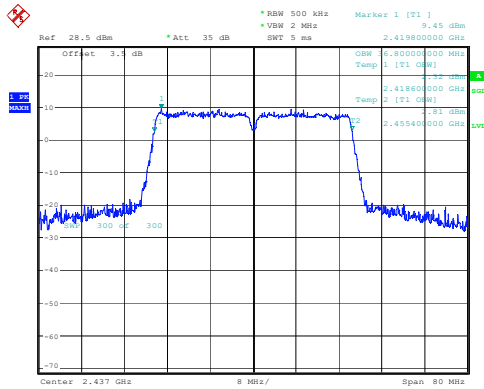
802.11n40_2437MHz
