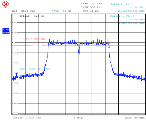
802.11n40_2422MHz
