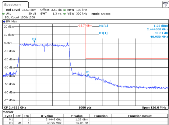
802.11ax40_2452MHz_RU_Full
