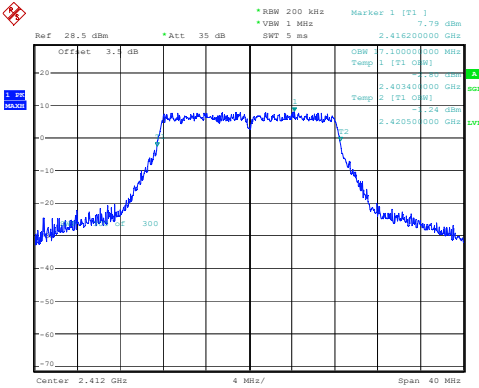
802.11g_2412MHz
