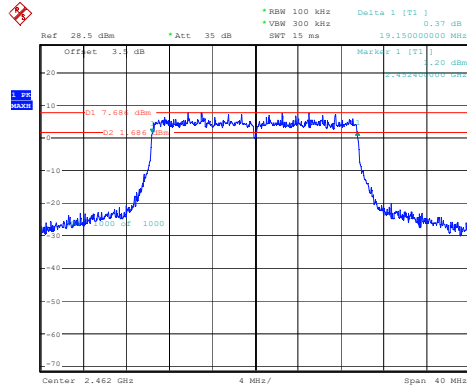
802.11ax20_2462MHz_RU_Full
