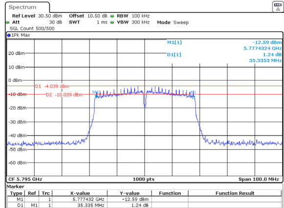
802.11ac40_5795MHz_Chain 1
