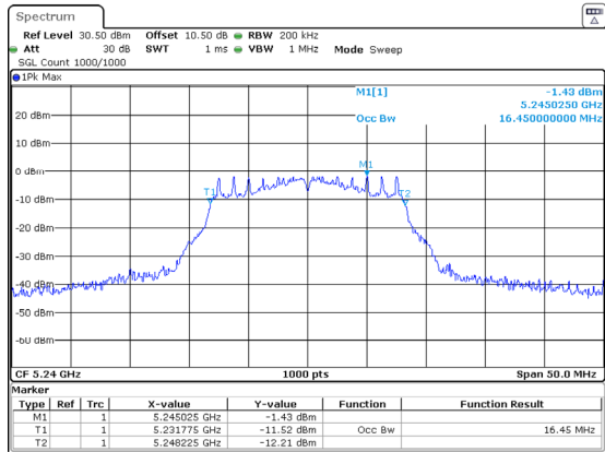
802.11a_5240MHz_Chain 1
