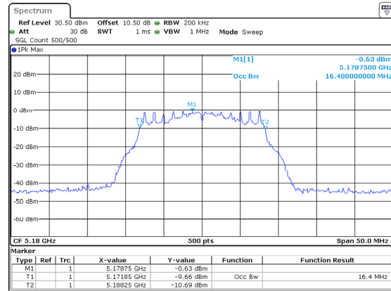
802.11a_5180MHz_Chain 2
