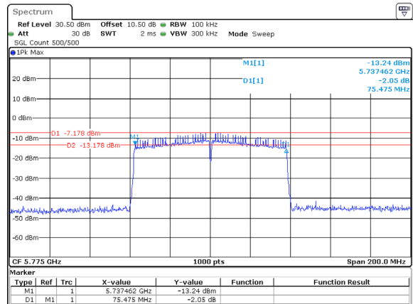
802.11ac80_5775MHz_Chain 2
