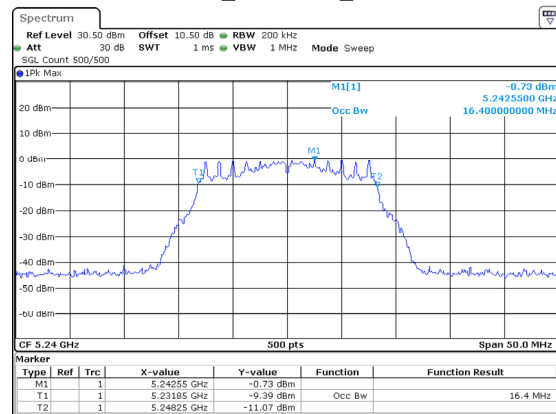
802.11a_5240MHz_Chain 2
