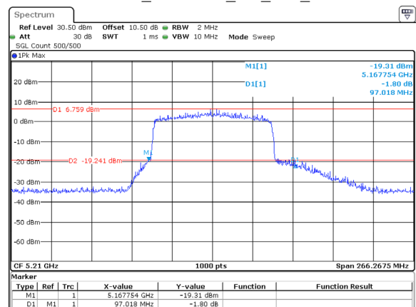
802.11ax80_5210MHz_RU_Full_Chain 2
