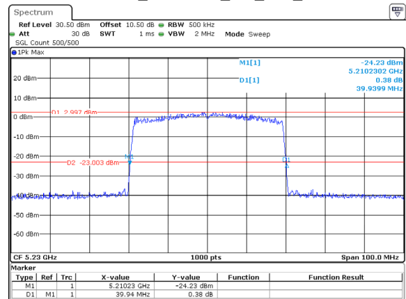
802.11ax40_5230MHz_RU_Full_Chain 2
