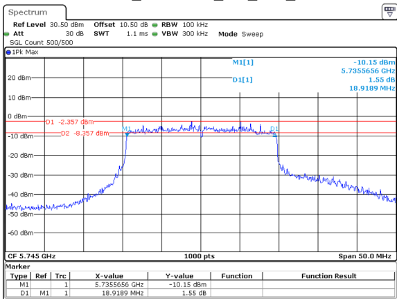
802.11ax20_5745MHz_RU_Full_Chain 2
