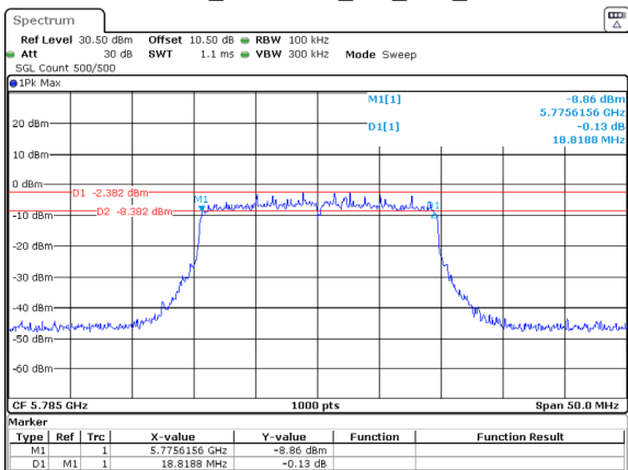
802.11ax20_5785MHz_RU_Full_Chain 1
