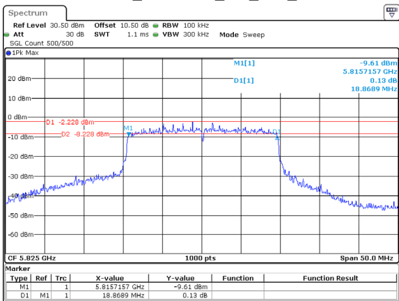
802.11ax20_5825MHz_RU_Full_Chain 2
