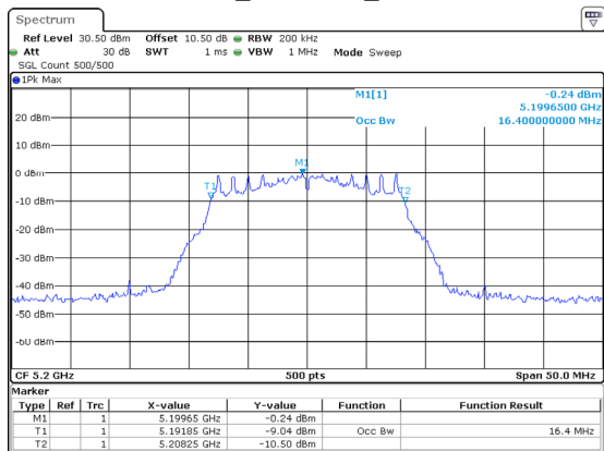
802.11a_5200MHz_Chain 2
