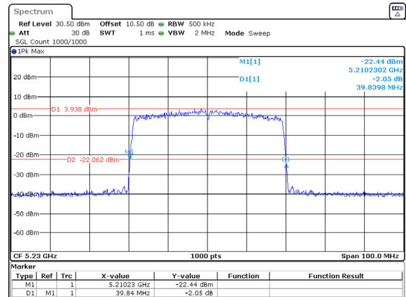
802.11ax40_5230MHz_RU_Full_Chain 1
