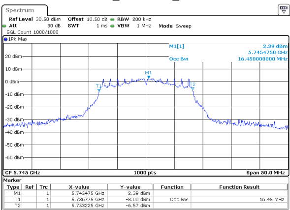
802.11a_5745MHz_Chain 1
