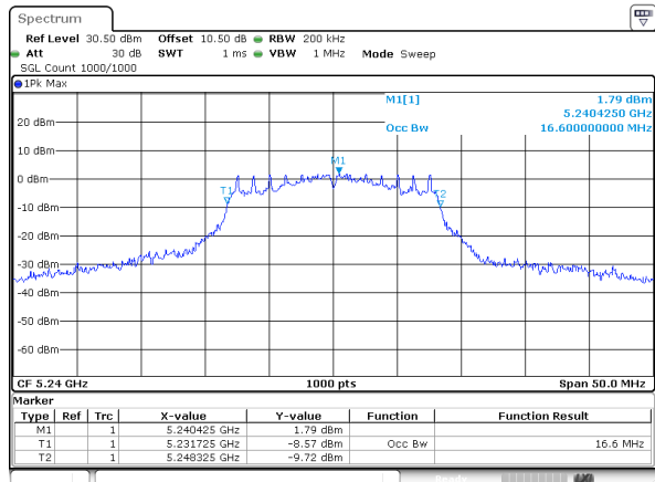
802.11a_5240MHz_Chain 0
