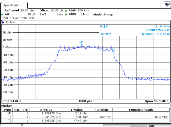
802.11a_5240MHz_Chain 1
