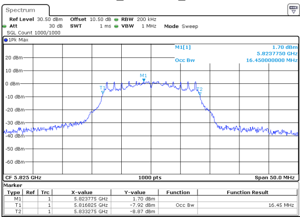
802.11a_5825MHz_Chain 1
