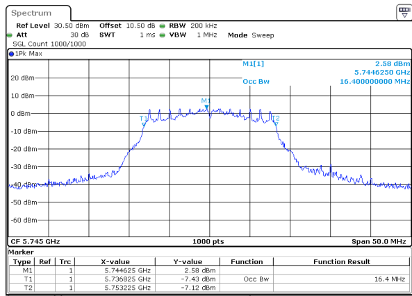
802.11a_5745MHz_Chain 0
