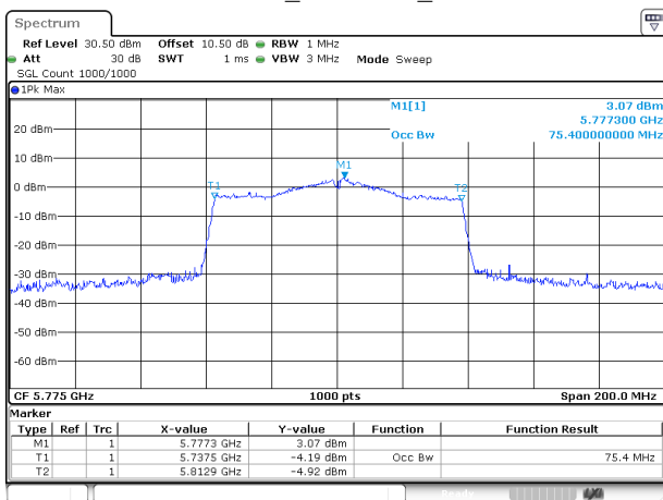
802.11ac80_5775MHz_Chain 0
