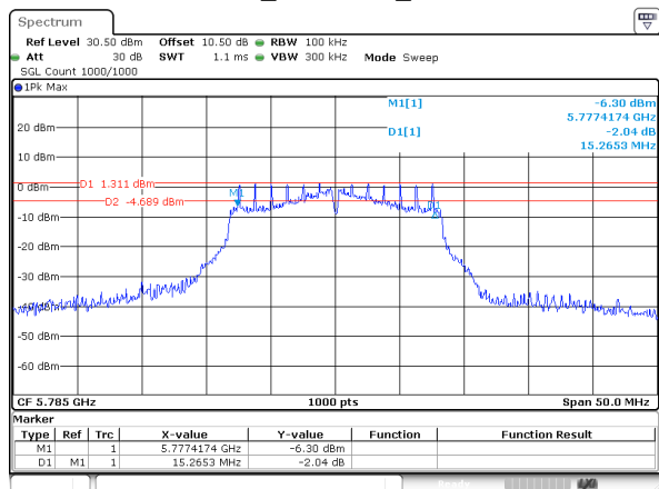
802.11a_5785MHz_Chain 1
