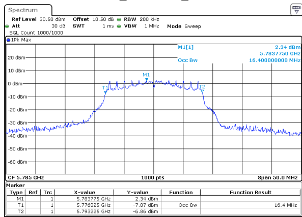
802.11a_5785MHz_Chain 1
