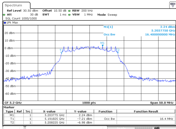
802.11a_5200MHz_Chain 1
