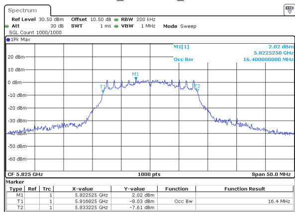
802.11a_5825MHz_Chain 0
