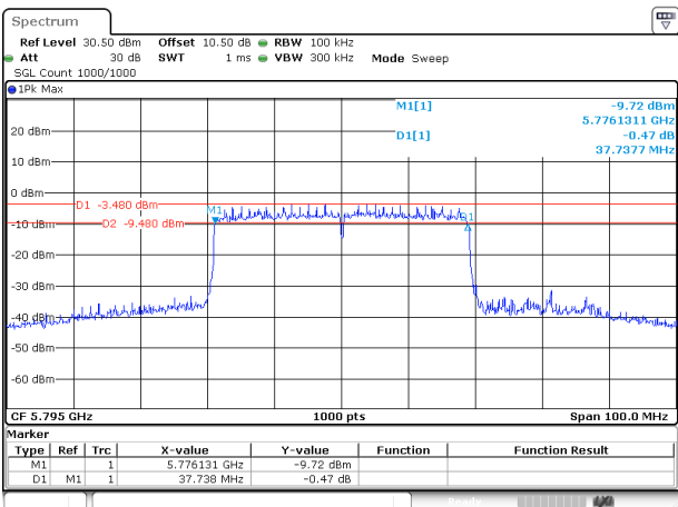
802.11ax40_5795MHz_RU_Full_Chain 1
