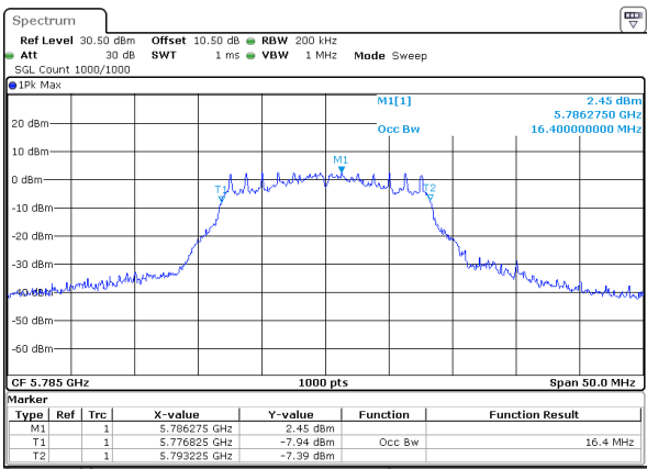
802.11a_5785MHz_Chain 0
