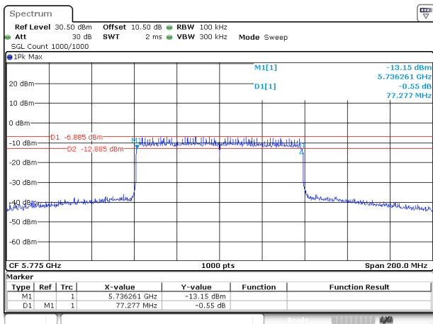
802.11ax80_5775MHz_RU_Full_Chain 0
