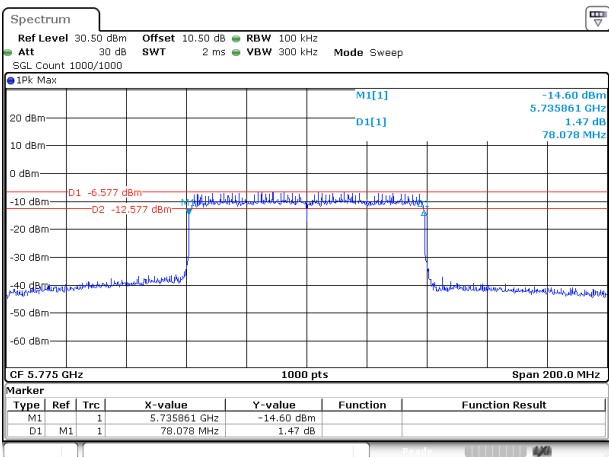
802.11ax80_5775MHz_RU_Full_Chain 1
