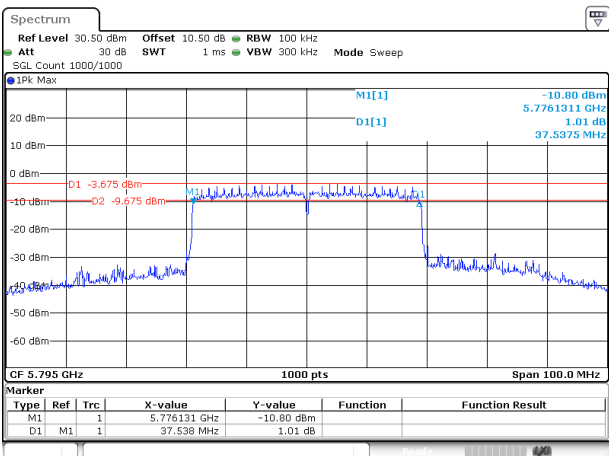
802.11ax40_5795MHz_RU_Full_Chain 0
