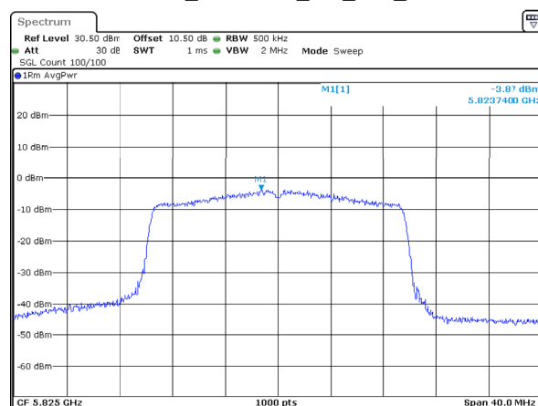
802.11ax20_5825MHz_RU_Full_Chain 2
