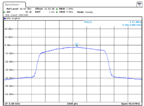
802.11ax20_5580MHz_RU_Full_Chain 1
