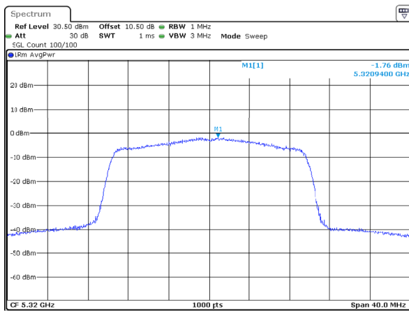
802.11ax20_5320MHz_RU_Full_Chain 1
