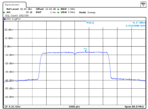
802.11ax40_5310MHz_RU_Full_Chain 1
