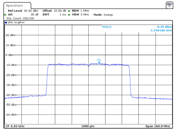
802.11ax80_5530MHz_RU_Full_Chain 2
