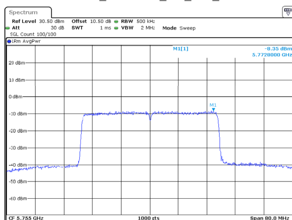
802.11ax40_5755MHz_RU_Full_Chain 1
