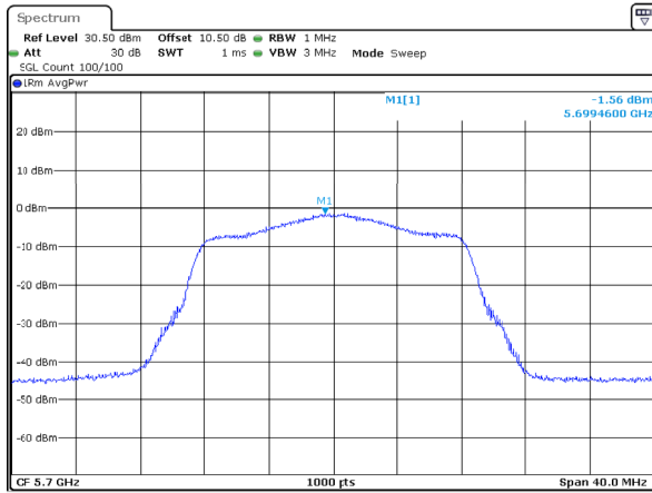
802.11a_5700MHz_Chain 2
