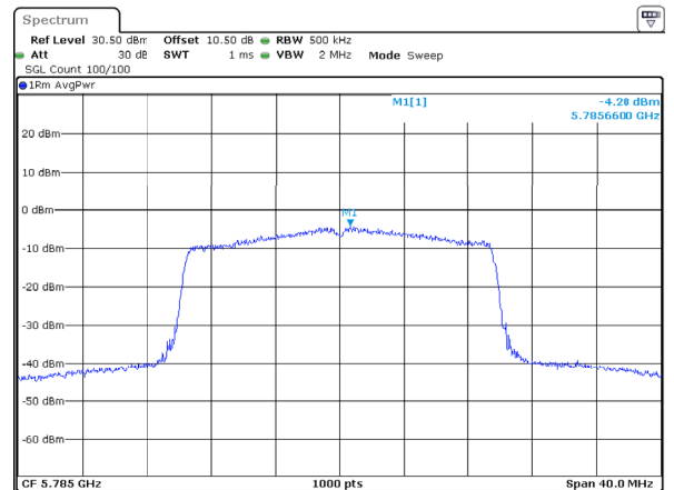
802.11ax20_5785MHz_RU_Full_Chain 1
