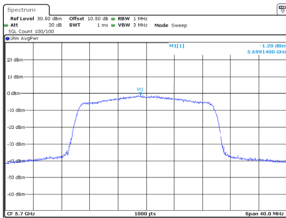
802.11ax20_5700MHz_RU_Full_Chain 1
