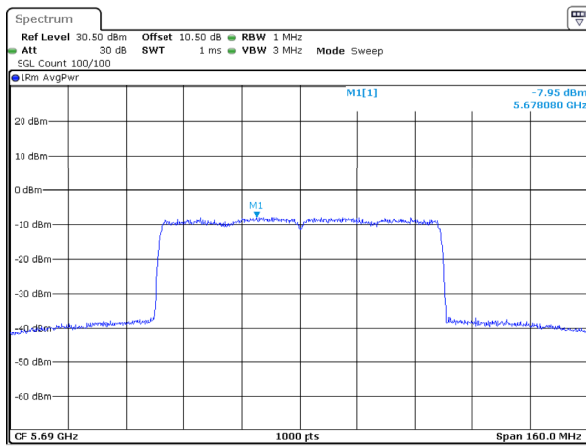
802.11ax80_5690MHz_RU_Full_Chain 1
