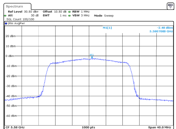
802.11ax20_5580MHz_RU_Full_Chain 2
