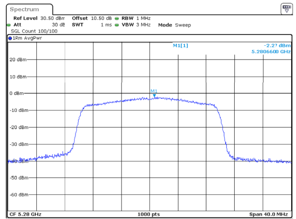
802.11ax20_5280MHz_RU_Full_Chain 1
