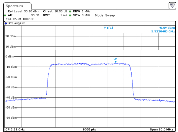
802.11ax40_5310MHz_RU_Full_Chain 2
