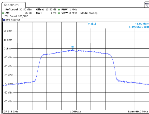
802.11ax20_5500MHz_RU_Full_Chain 1
