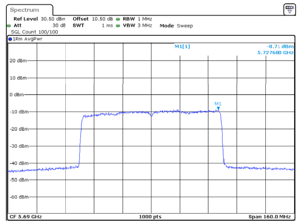
802.11ax80_5690MHz_RU_Full_Chain 2
