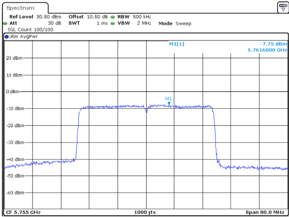
802.11ax40_5755MHz_RU_Full_Chain 2
