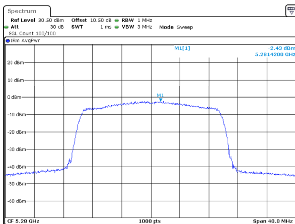
802.11ax20_5280MHz_RU_Full_Chain 2
