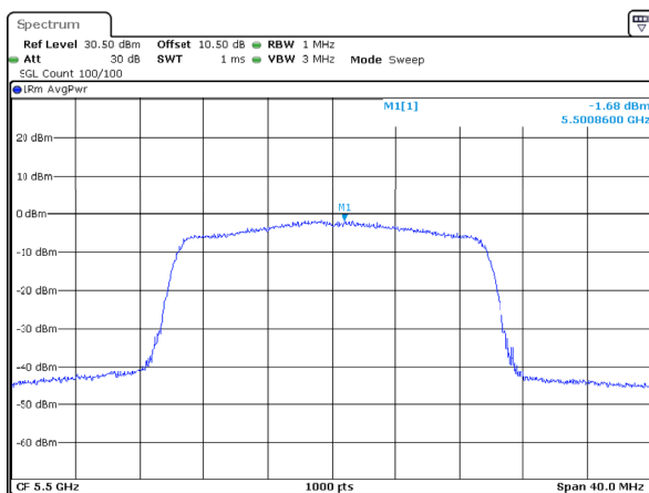
802.11ax20_5500MHz_RU_Full_Chain 2
