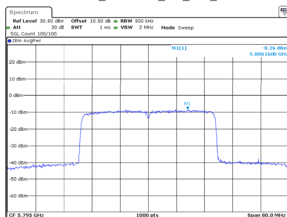
802.11ax40_5795MHz_RU_Full_Chain 1
