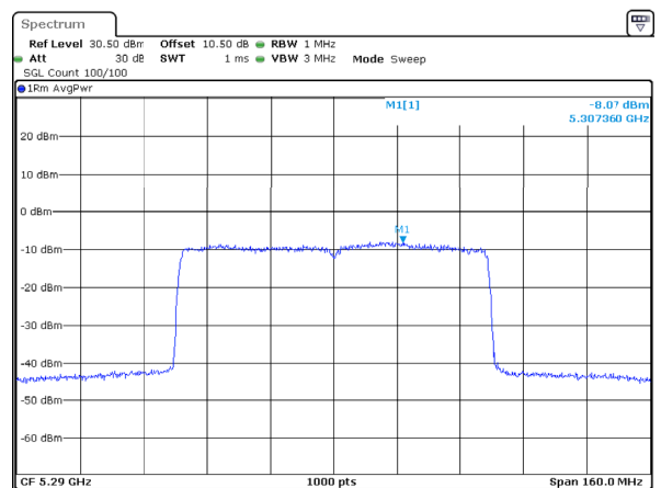
802.11ax80_5290MHz_RU_Full_Chain 2
