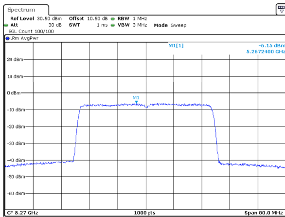
802.11ax40_5270MHz_RU_Full_Chain 2
