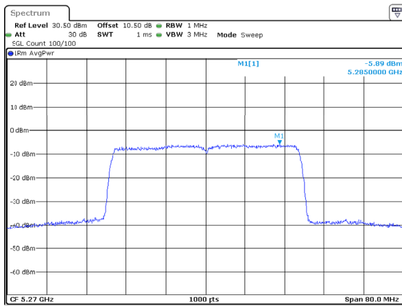
802.11ax40_5270MHz_RU_Full_Chain 1
