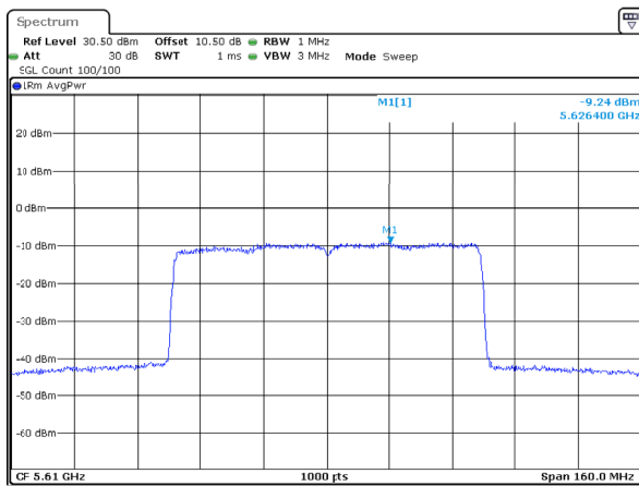
802.11ax80_5610MHz_RU_Full_Chain 2
