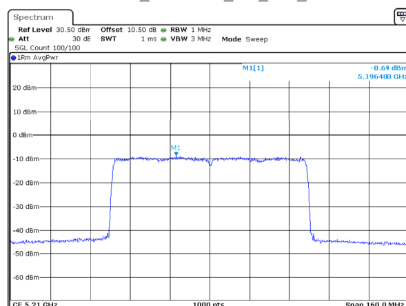
802.11ax80_5210MHz_RU_Full_Chain 2
