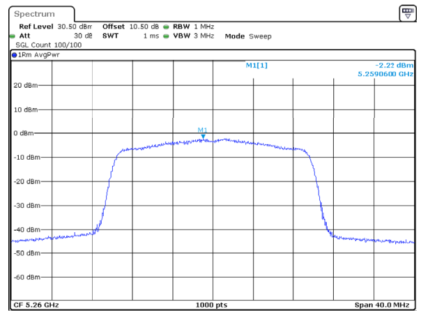
802.11ax20_5260MHz_RU_Full_Chain 2
