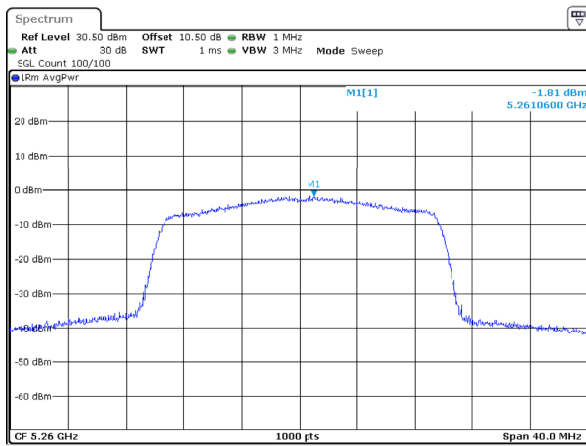
802.11ax20_5260MHz_RU_Full_Chain 1
