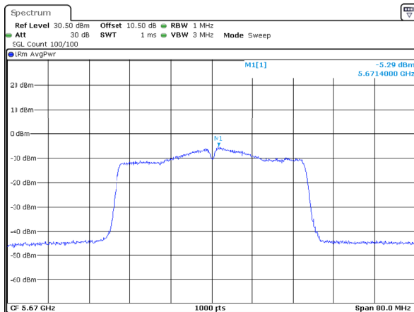
802.11ac40_5670MHz_Chain 2
