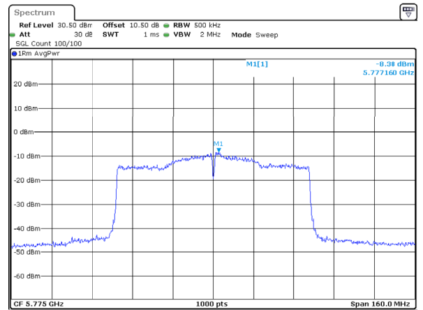
802.11ac80_5775MHz_Chain 2
