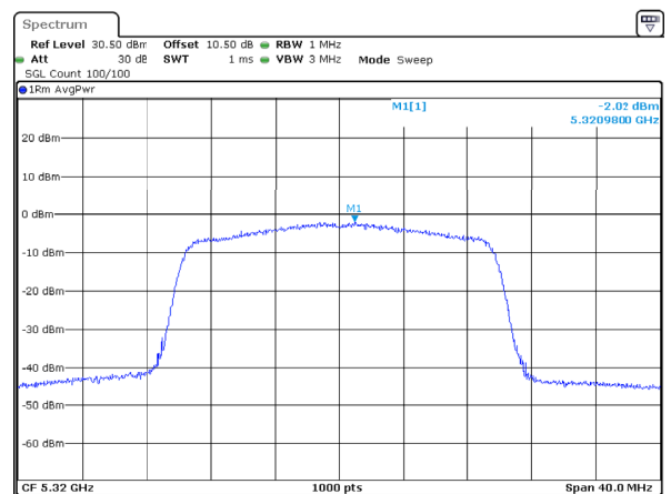
802.11ax20_5320MHz_RU_Full_Chain 2
