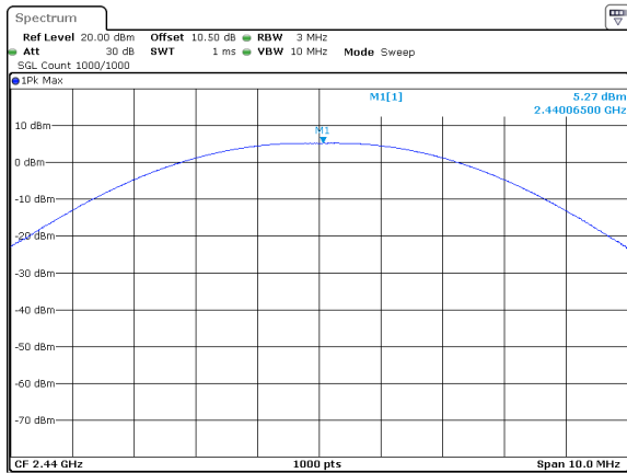
BLE_2M_Middle_Channel
