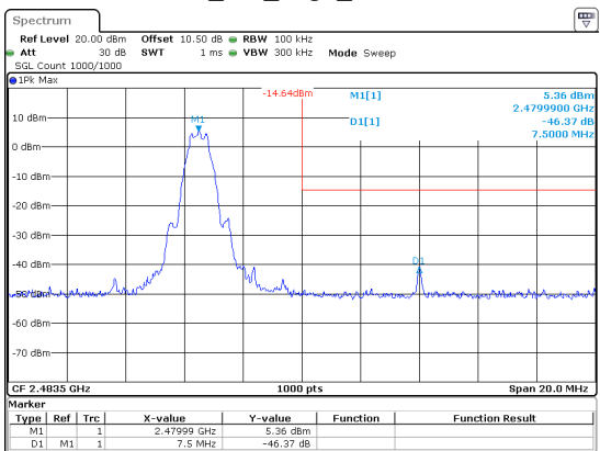
BLE_1M_High_Channel
