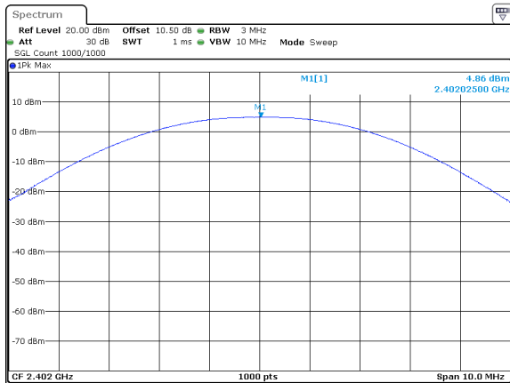
BLE_1M_Low_Channel
