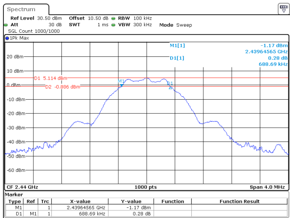
BLE_1M_Middle_Channel
