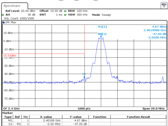
BLE_1M_Low_Channel
