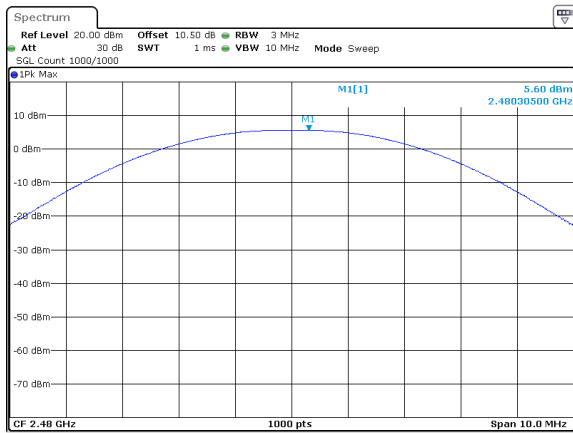
BLE_1M_High_Channel
