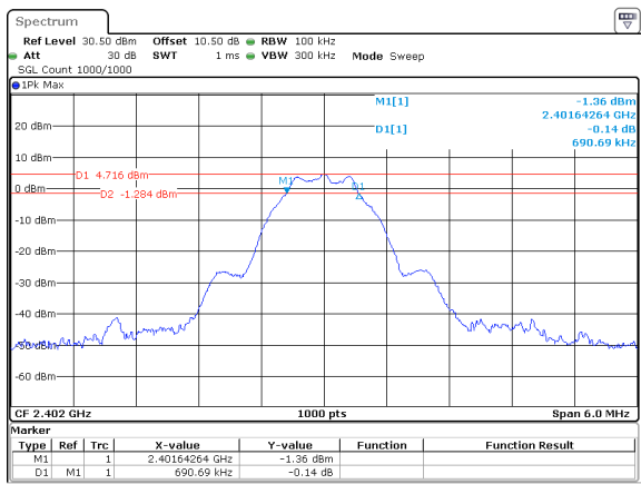
BLE_2M_Low_Channel
