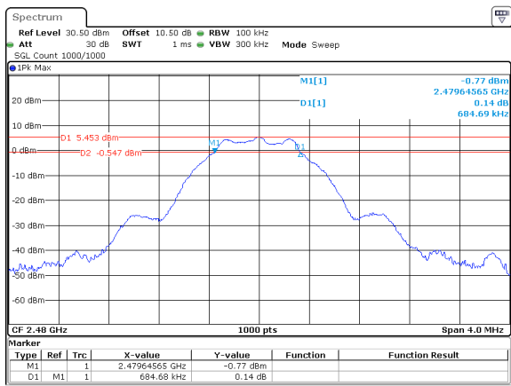
BLE_1M_High_Channel
