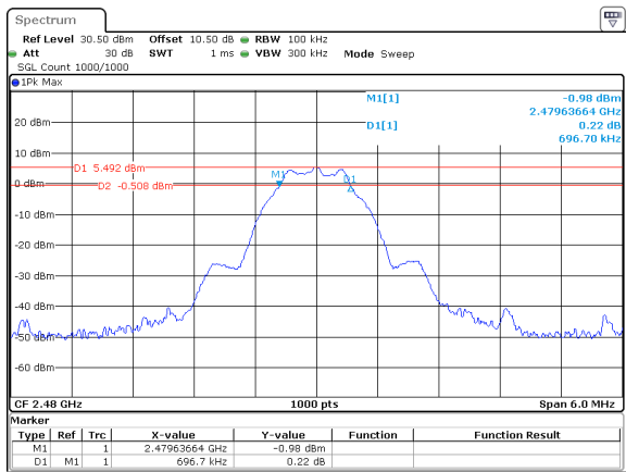
BLE_2M_High_Channel
