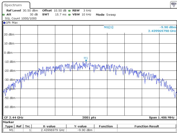
BLE_2M_Middle_Channel
