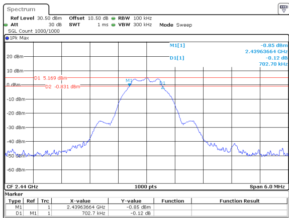
BLE_2M_Middle_Channel
