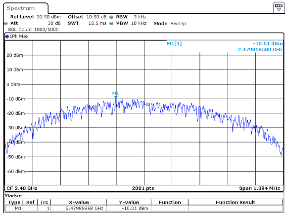
BLE_2M_High_Channel
