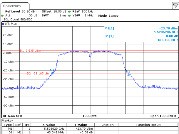
802.11ac40_5550MHz_Chain 0
