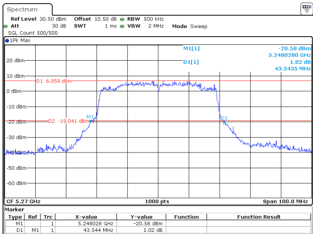
802.11ax40_5270MHz_RU_Full_Chain 0
