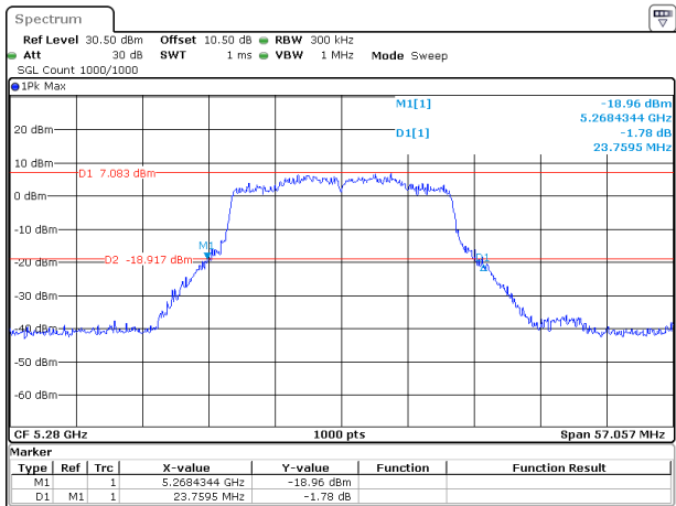
802.11ax20_5280MHz_RU_Full_Chain 1
