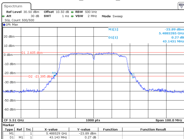
802.11ac40_5510MHz_Chain 0
