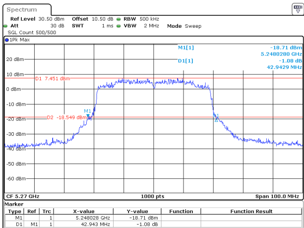
802.11ax40_5270MHz_RU_Full_Chain 1
