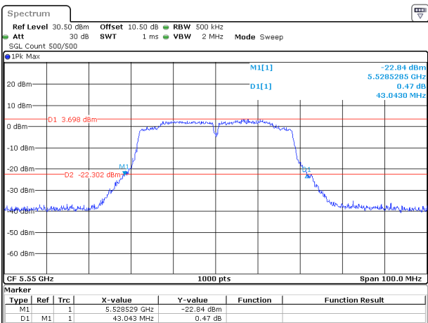
802.11ac40_5550MHz_Chain 1
