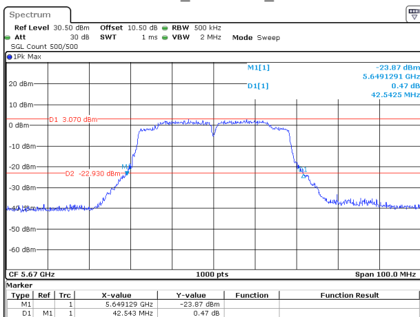
802.11ac40_5670MHz_Chain 0
