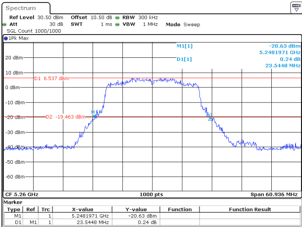
802.11ax20_5260MHz_RU_Full_Chain 1
