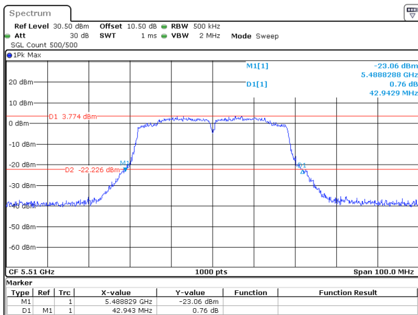
802.11ac40_5510MHz_Chain 1
