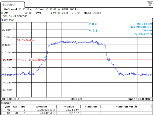
802.11ax40_5310MHz_RU_Full_Chain 0
