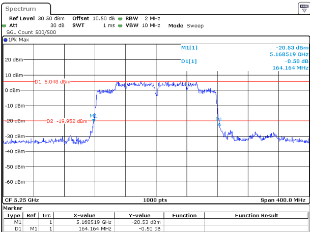
802.11ac160_5250MHz_Chain 0
