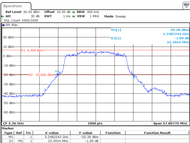
802.11ax20_5260MHz_RU_Full_Chain 0
