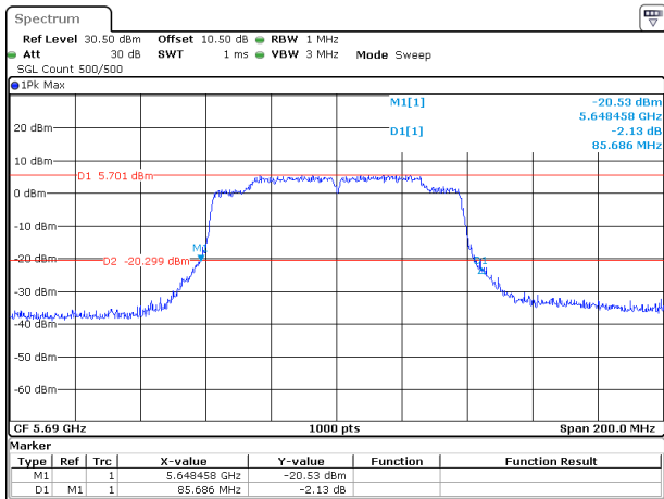
802.11ac80_5690MHz_Chain 0
