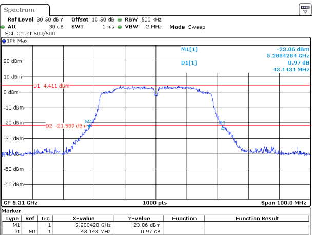
802.11ac40_5310MHz_Chain 0
