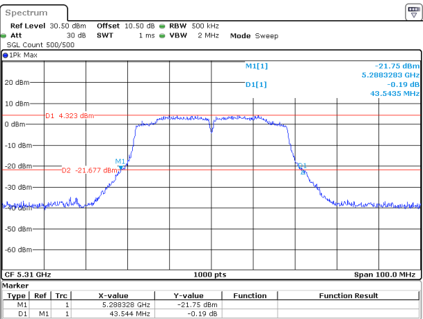
802.11ac40_5310MHz_Chain 1
