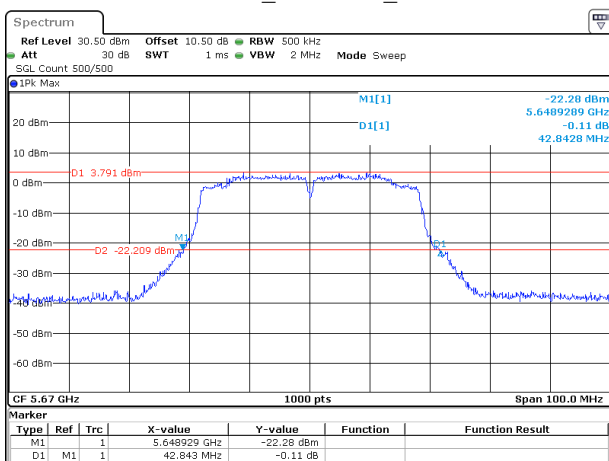
802.11ac40_5670MHz_Chain 1
