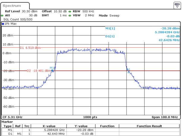
802.11ax40_5310MHz_RU_Full_Chain 1
