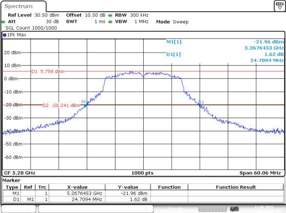
802.11a_5280MHz_Chain 0
