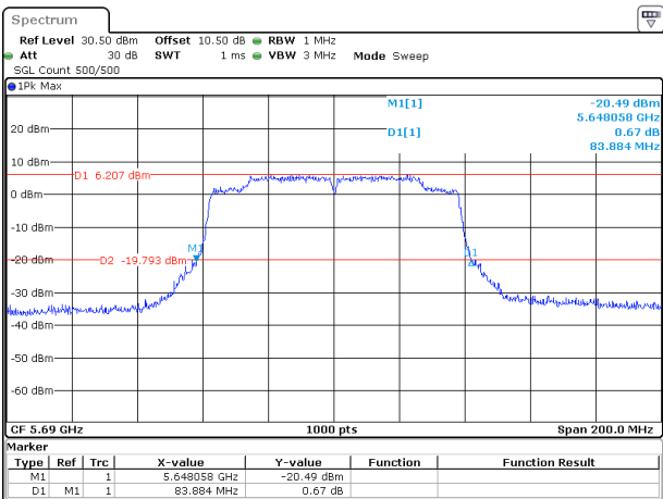
802.11ac80_5690MHz_Chain 1
