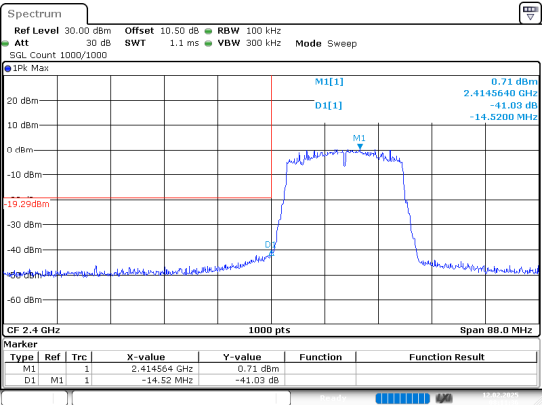
802.11ax20_2412MHz_Chain 0
