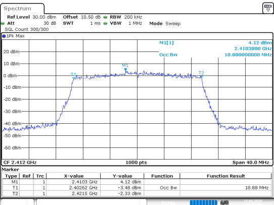
802.11ax20_2412MHz_Chain 0
