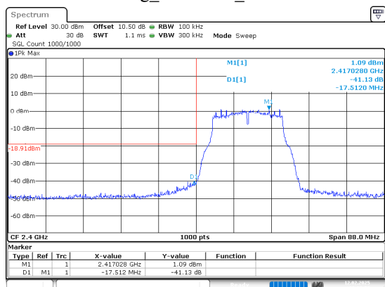
802.11g_2412MHz_Chain 0
