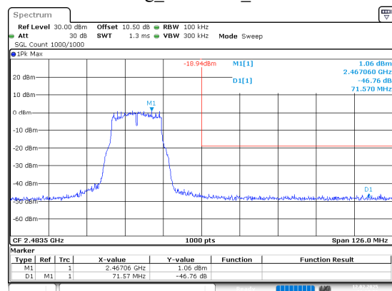
802.11g_2462MHz_Chain 0
