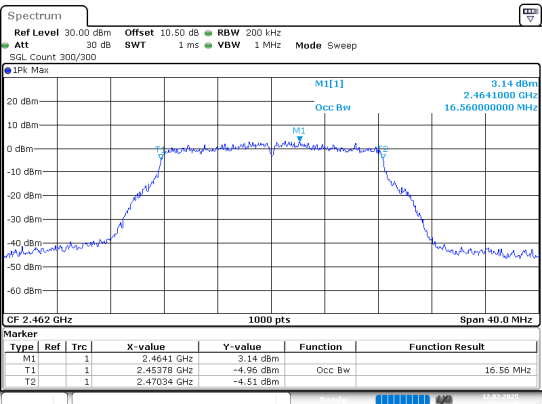
802.11g_2462MHz_Chain 0
