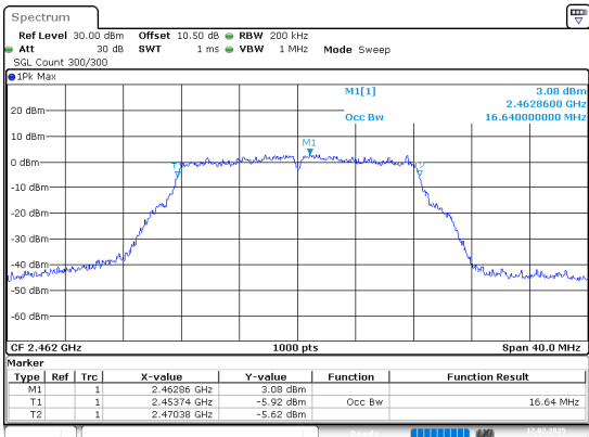
802.11g_2462MHz_Chain 1
