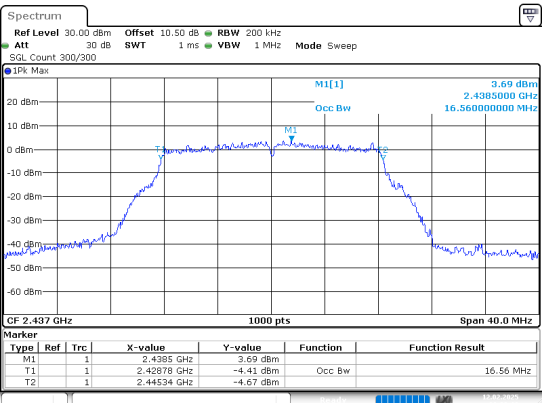
802.11g_2437MHz_Chain 1
