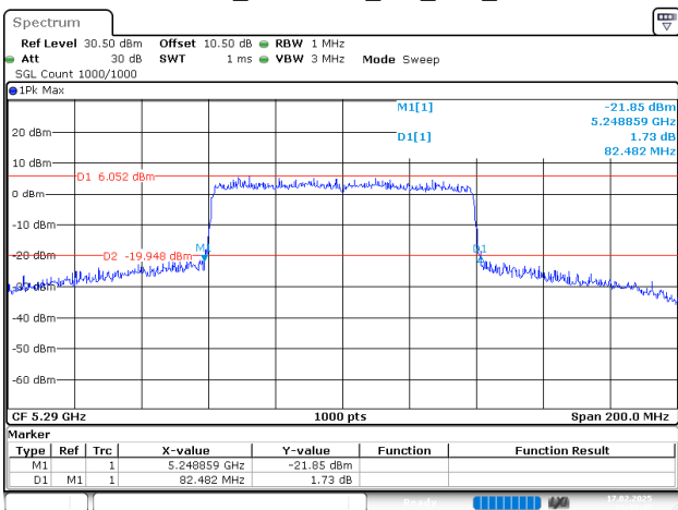
802.11ax80_5290MHz_RU_Full_Chain 1
