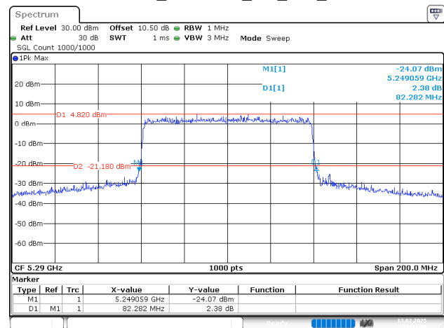
802.11ax80_5290MHz_RU_Full_Chain 0
