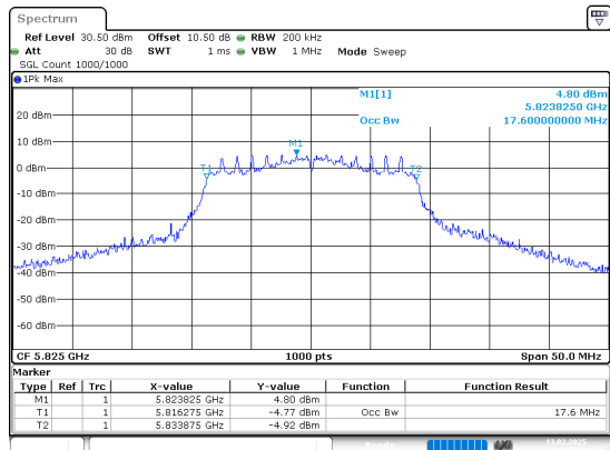
802.11n20_5825MHz_Chain 0
