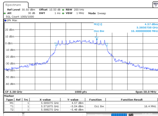
802.11a_5580MHz_Chain 0
