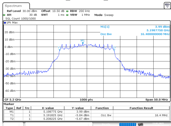
802.11a_5200MHz_Chain 1
