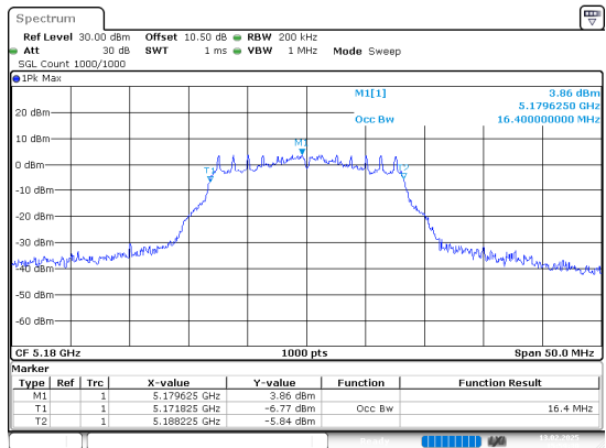
802.11a_5180MHz_Chain 1
