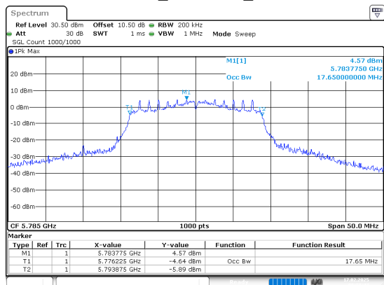
802.11n20_5785MHz_Chain 1
