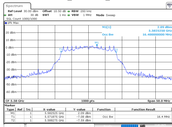
802.11a_5580MHz_Chain 1
