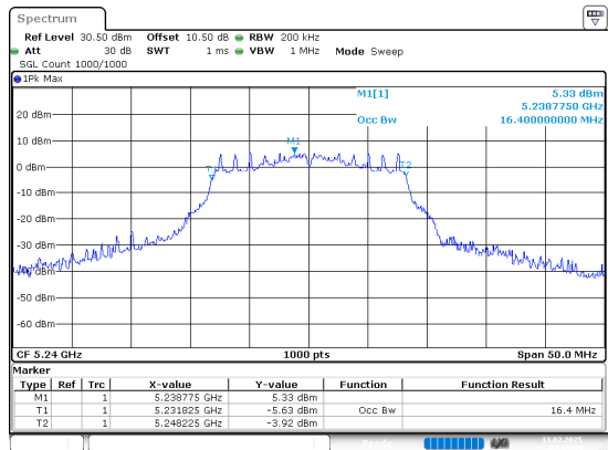
802.11a_5240MHz_Chain 0
