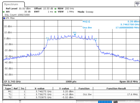
802.11n20_5745MHz_Chain 1
