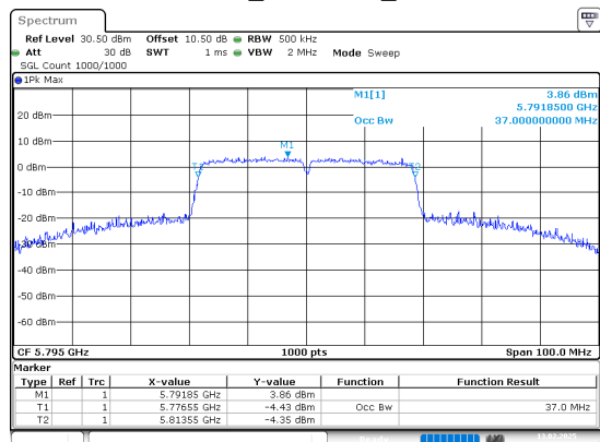
802.11n40_5795MHz_Chain 0
