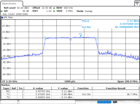
802.11n40_5550MHz_Chain 1
