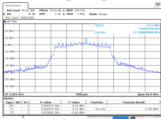
802.11n20_5825MHz_Chain 1
