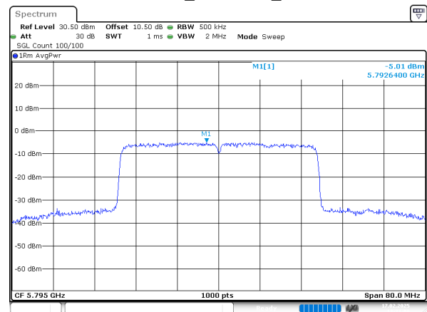
802.11ax40_5795MHz_Chain 1
