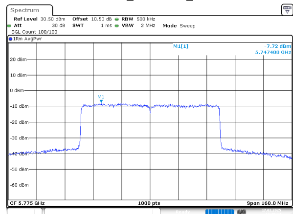
802.11ax80 5775MHz Chain 1
