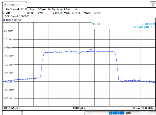
802.11ax40_5550MHz_Chain 1
