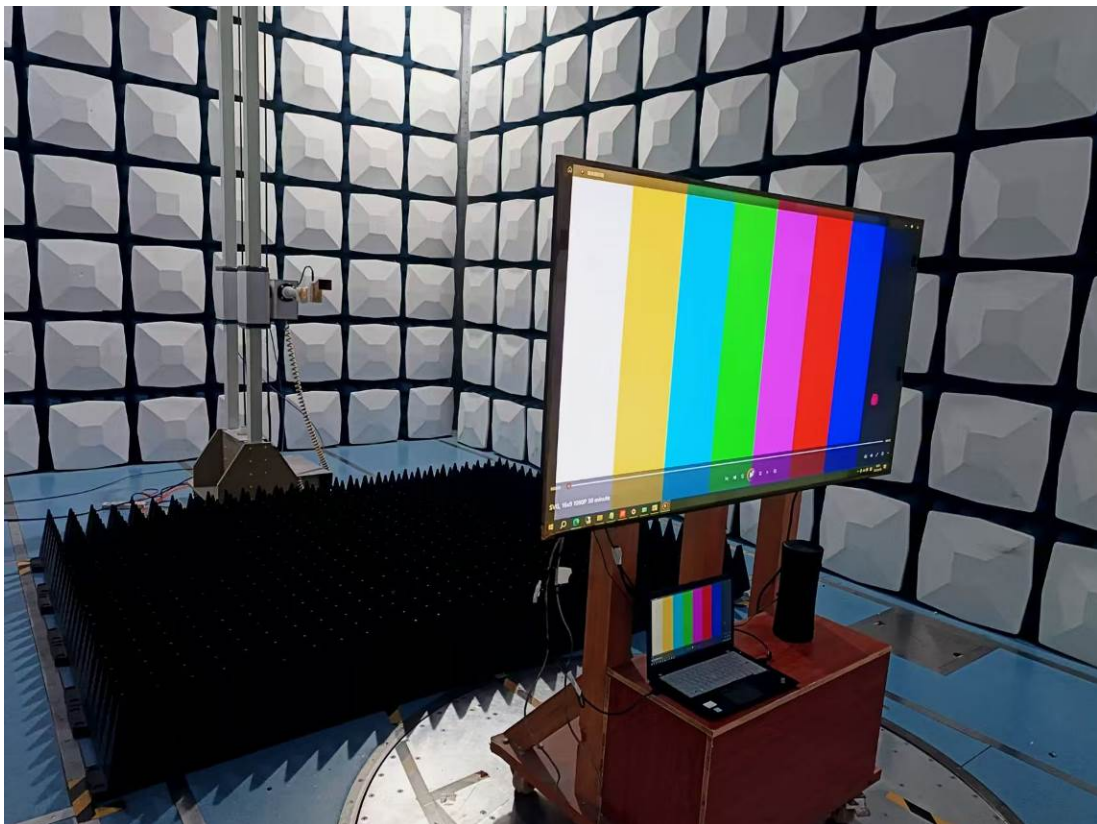
Radiated Emission 18-25GHz View
