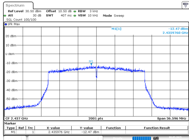
802.11ax20_2437MHz_RU_Full_Chain 0
