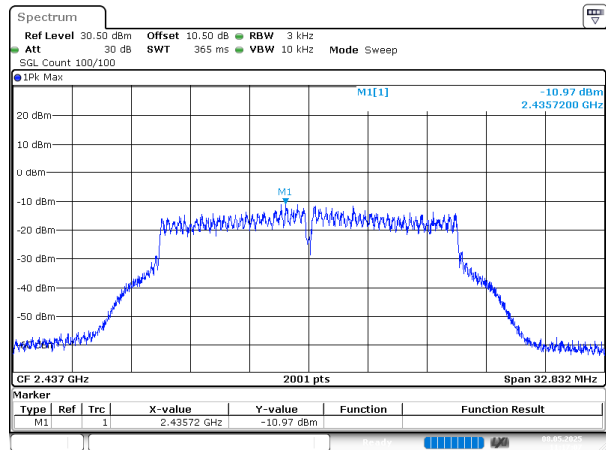
802.11g_2437MHz_Chain 0
