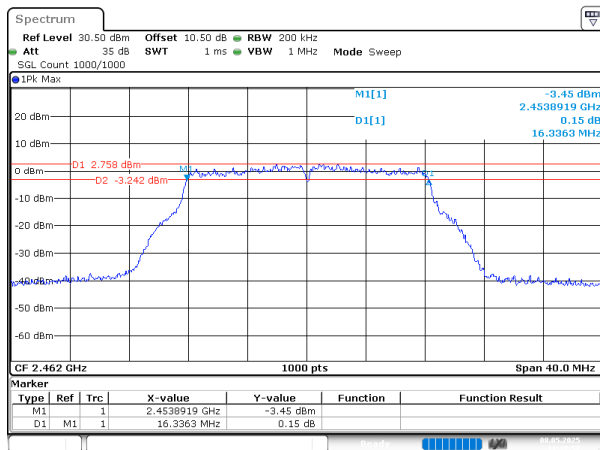
802.11g_2462MHz_Chain 0
