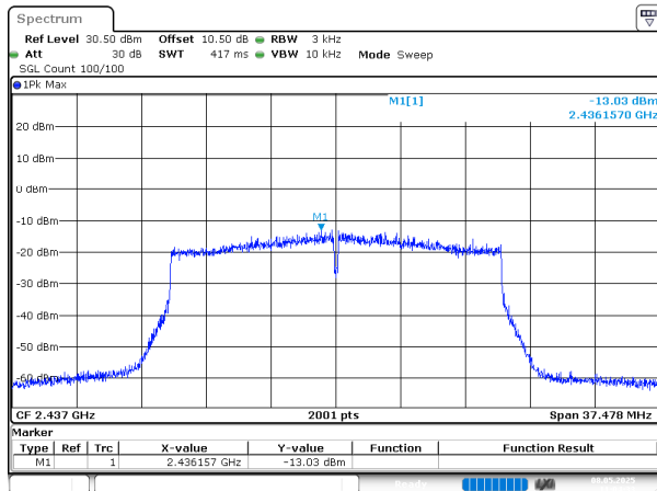
802.11ax20_2437MHz_RU_Full_Chain 1
