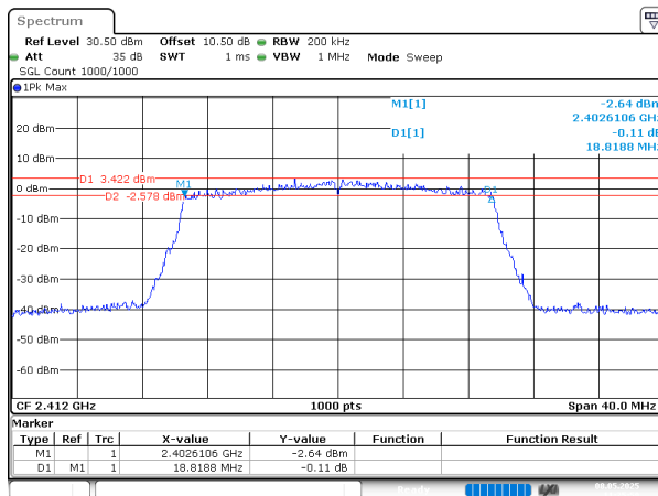
802.11ax20_2412MHz_RU_Full_Chain 0
