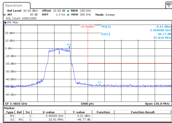
802.11g_2462MHz_Chain 0
