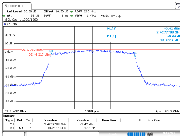
802.11ax20_2437MHz_RU_Full_Chain 1
