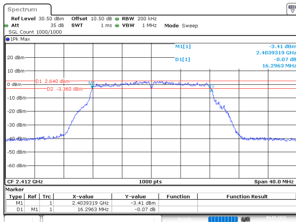
802.11g_2412MHz_Chain 0
