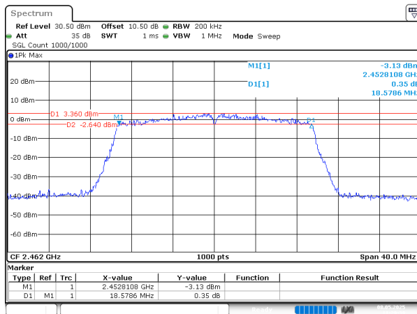
802.11ax20_2462MHz_RU_Full_Chain 0
