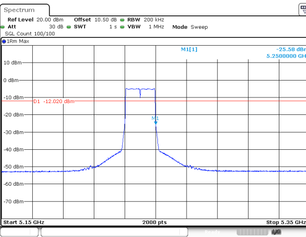
802.11ax20_5240MHz_RU_FULL
