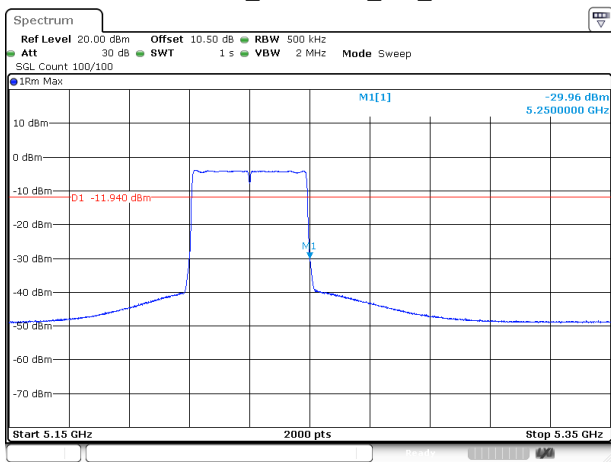
802.11ax40_5230MHz_RU_FULL
